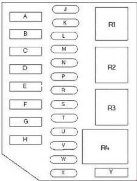
Lincoln Town Car – fuse box diagram – engine
