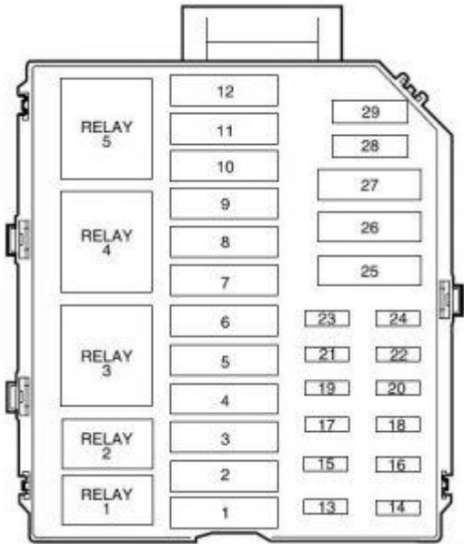
compartment diagram – engine compartment
