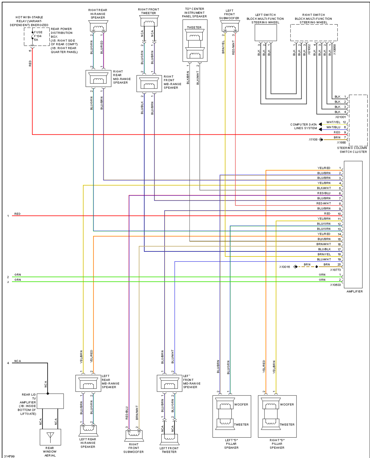
Fig. 111: Radio Circuit, W/ Top HIFI Radio (3 of 3)
