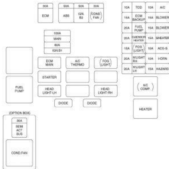
Isuzu Axim – fuse box diagram
