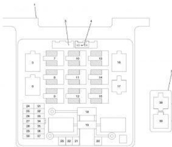
Isuzu Axim – fuse box diagram – engine compartment
