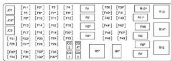
Buick Lucerne – fuse box – rear underseat
