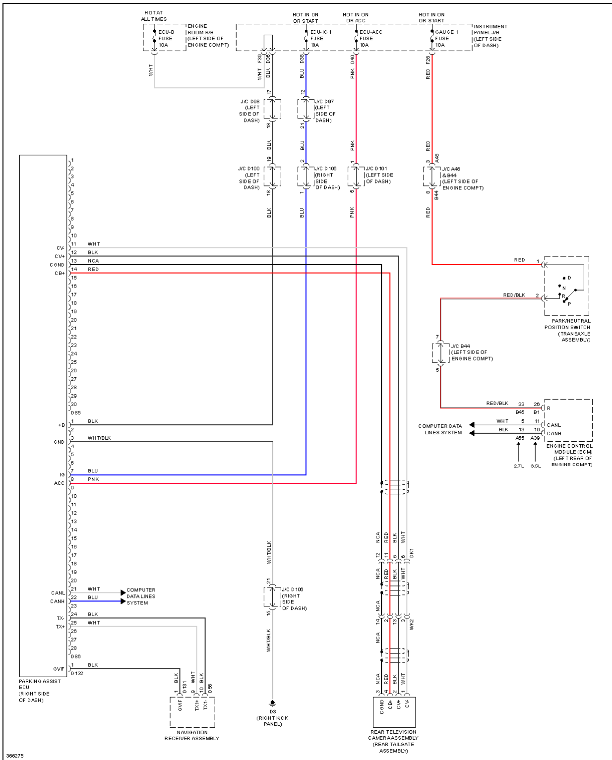
Fig. 65: Parking Assistant Circuit
