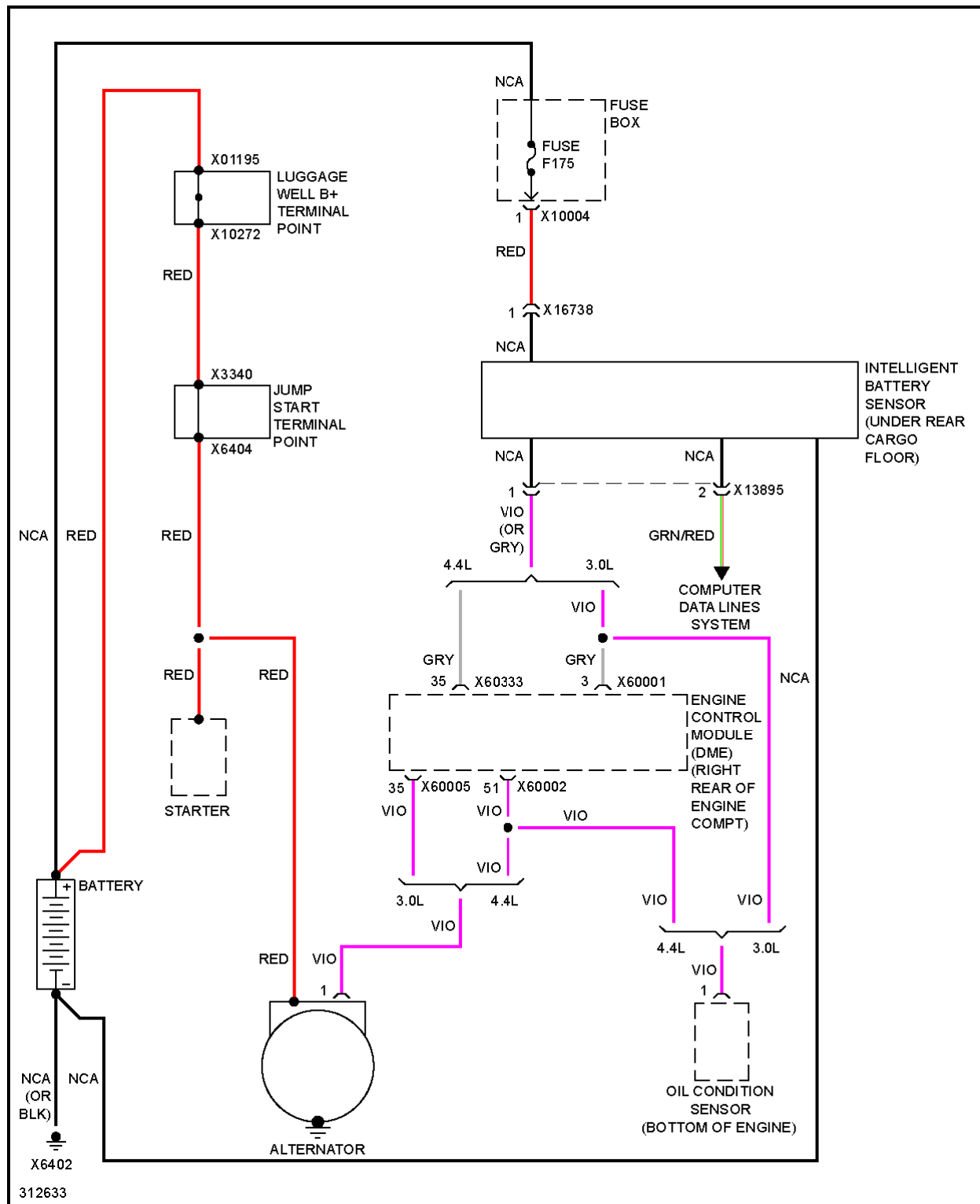
Fig. 118: Charging Circuit
