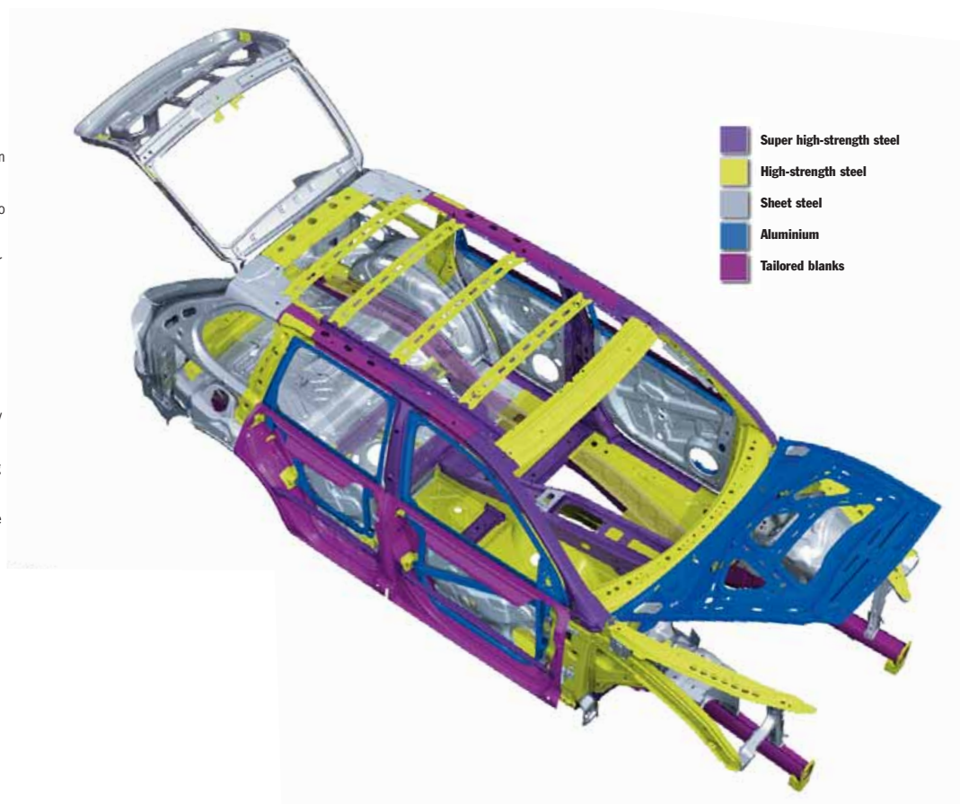
Passive safety: bodyshell
