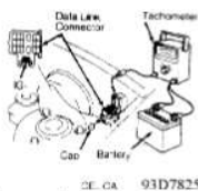
Fig. 3: Connecting Tachometer Courtesy of Toyota Motor Sales, U.S.A., Inc.
