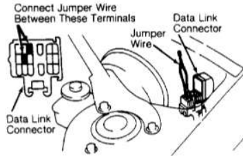
Fig. 4: Installing Jumper Wire Data Link Connector Terminals Courtesy of Toyota Motor Sales, U.S.A., Inc.
