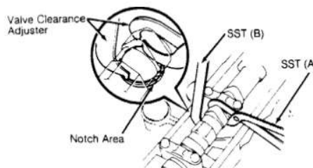
Fig. 2: Removing Valve Clearance Adjusting Shim Courtesy of Toyota Motor Sales, U.S.A., Inc.
