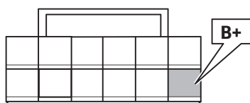
12 Pin Connector
