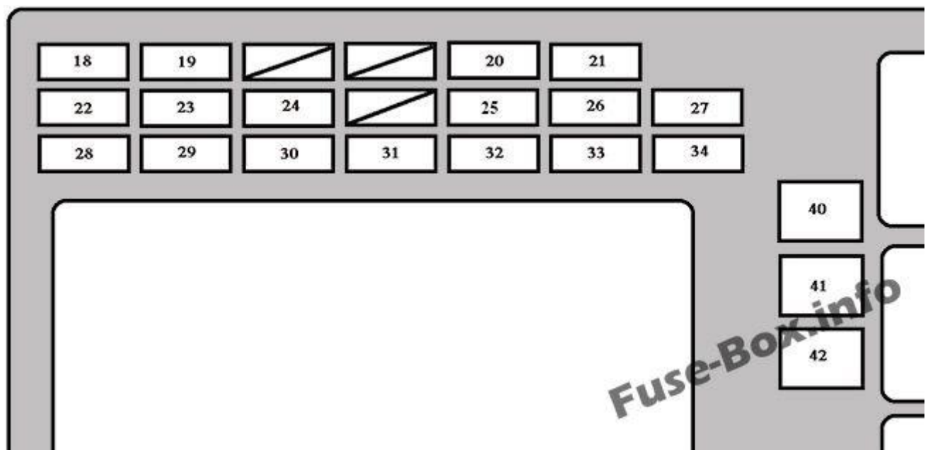
Fuse box diagram
