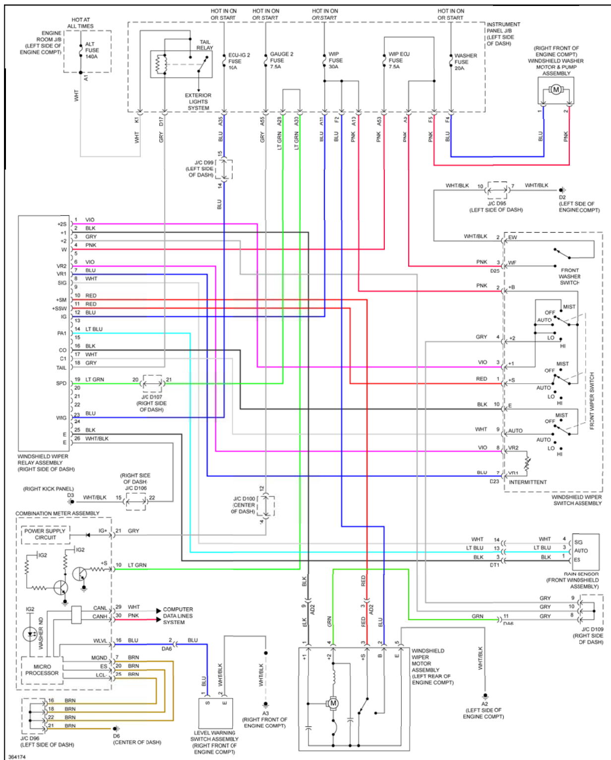
Fig. 126: Front Wiper/Washer Circuit, W/ Auto Wiper System
