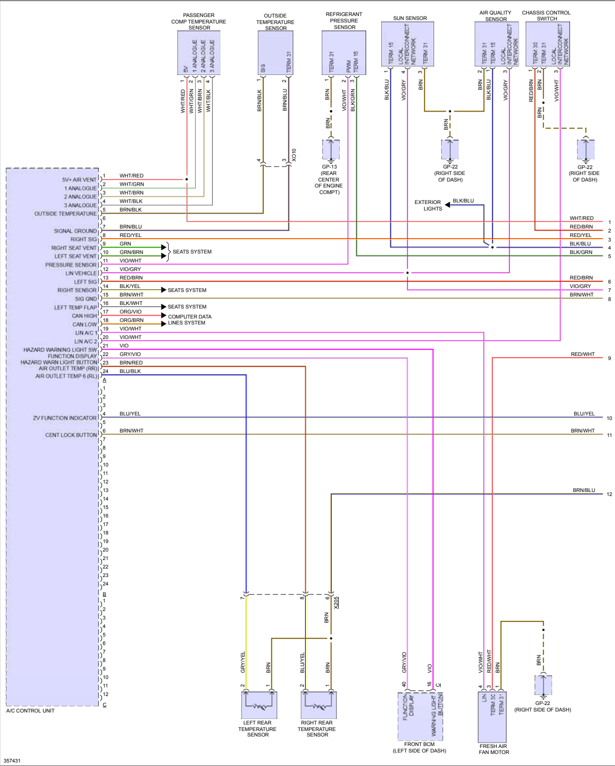
Fig 1: Automatic A/C Circuit (1 of 5)
