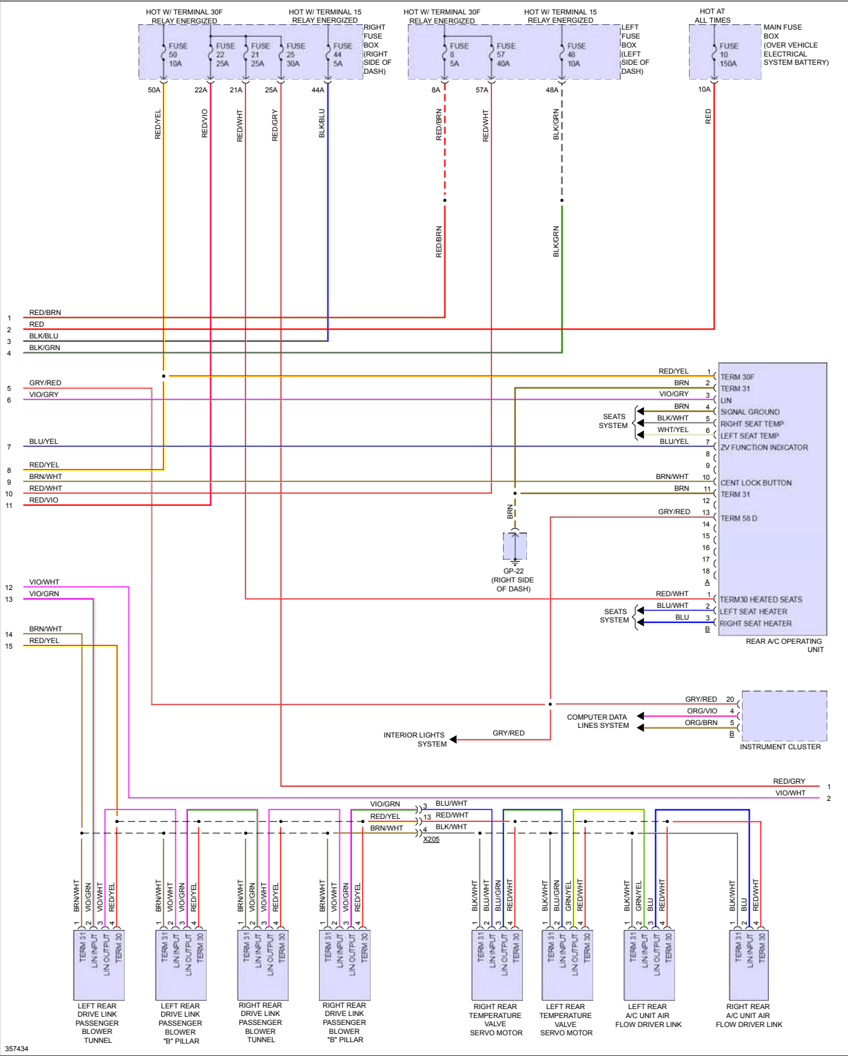
Fig 4: Automatic A/C Circuit (4 of 5)
