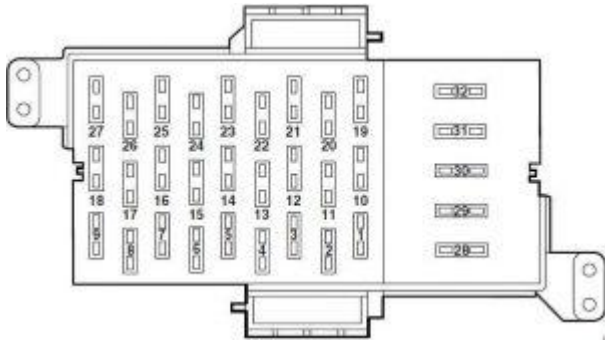
Mercury Grand Marquis – fuse box diagram – passenger compartment
