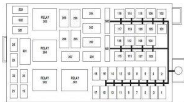
Mercury Grand Marquis – fuse box diagram – engine compartment
