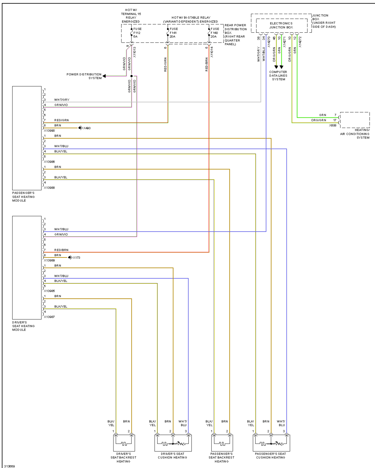
Fig. 92: Front Heated Seats Circuit, W/O Memory Seats
