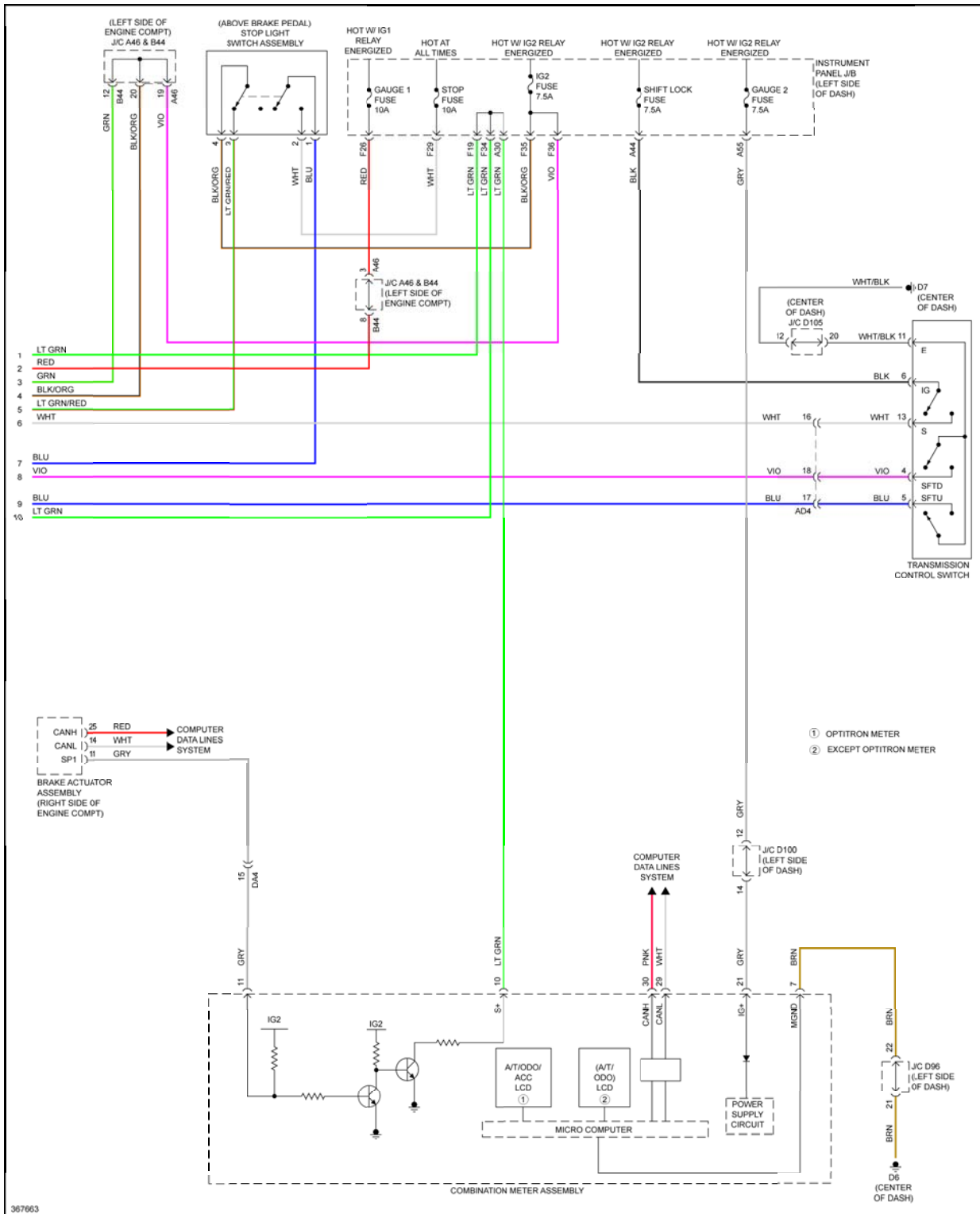
Fig. 112: 2.7L, A/T Circuit (2 of 2)
