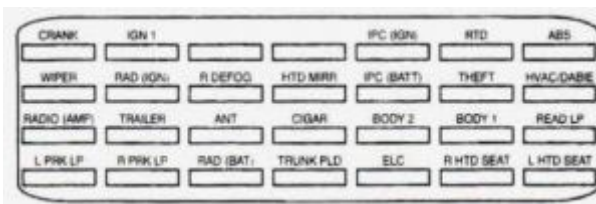
Cadillac Eldorado – fuse box diagram – trunk
