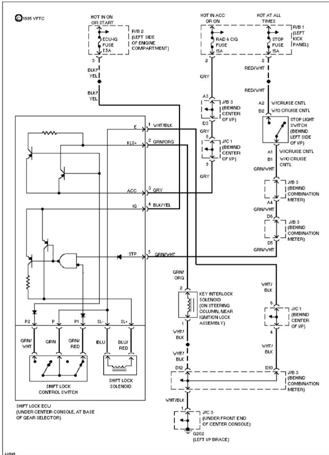
Fig. 10: Shift Interlock System Wiring Diagram (MR2) Courtesy of Toyota Motor Sales, U.S.A., Inc.
