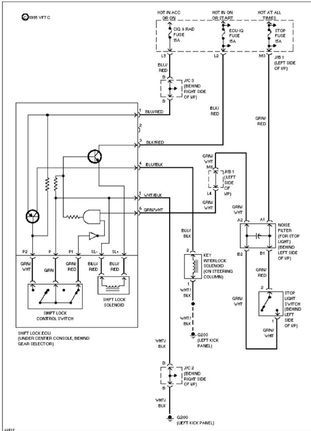
Fig. 6: Shift Interlock System Wiring Diagram (Camry) Courtesy of Toyota Motor Sales, U.S.A., Inc.
