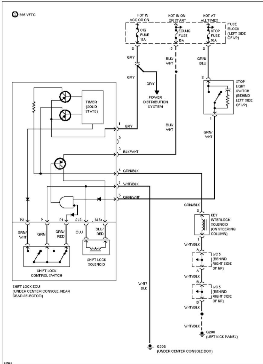
Fig. 9: Shift Interlock System Wiring Diagram (Land Cruiser) Courtesy of Toyota Motor Sales, U.S.A., Inc.
