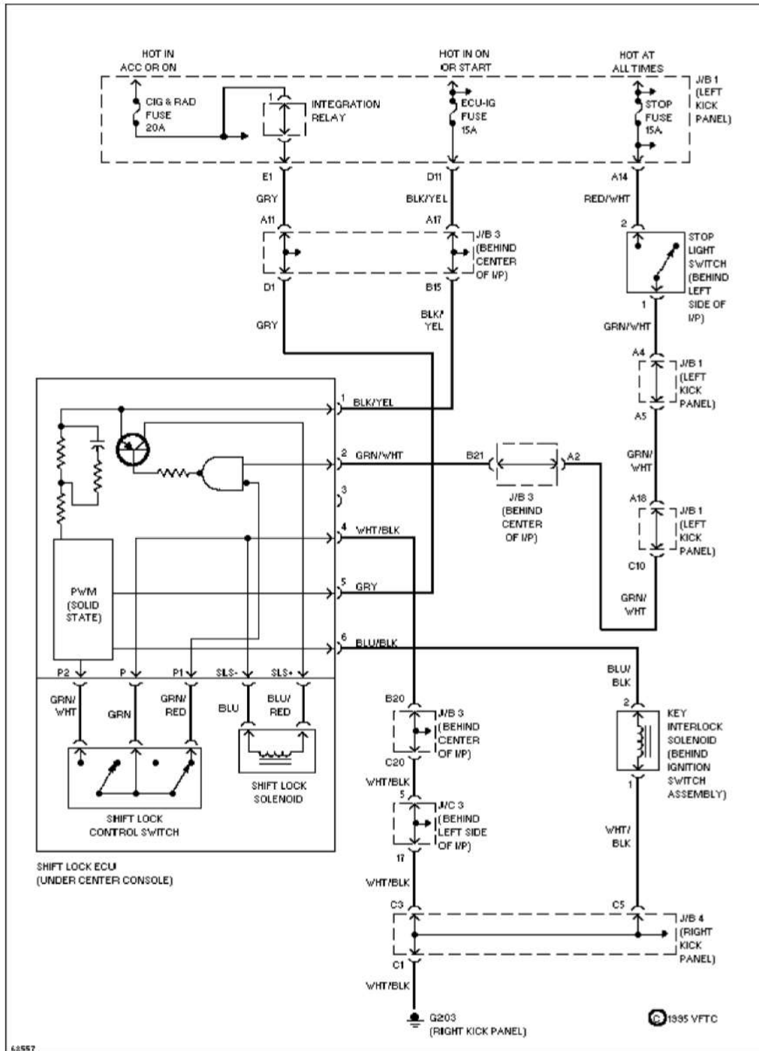
Fig. 8: Shift Interlock System Wiring Diagram (Corolla) Courtesy of Toyota Motor Sales, U.S.A., Inc.
