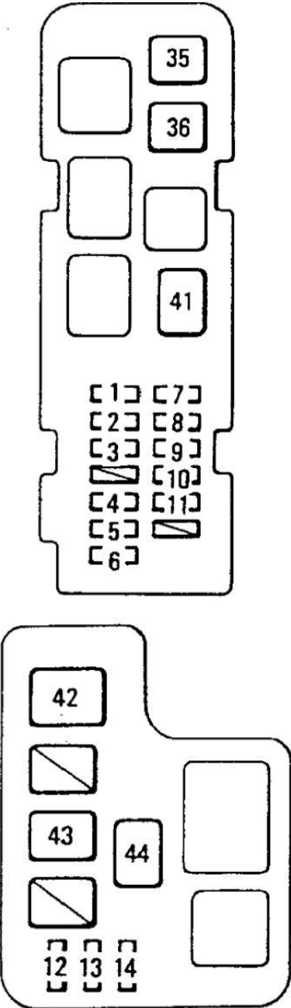
Fig. 7: Engine Compartment Main Fuse Identification (1994-95) Courtesy of Toyota Motor Sales, U.S.A., Inc.
