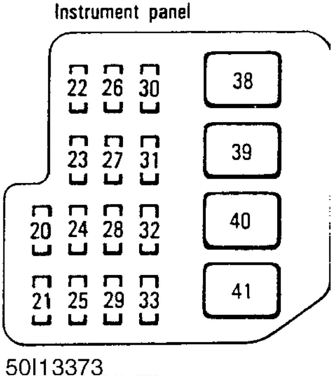
Fig. 12: Instrument Panel Identification (1996) Courtesy of Toyota Motor Sales, U.S.A., Inc.
