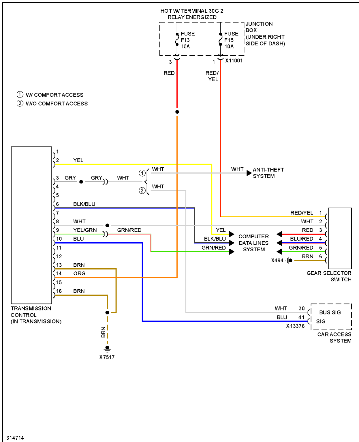
Fig. 126: 4.4L Twin Turbo, A/T Circuit
