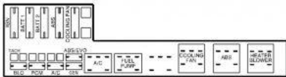
Pontiac Sunfire – fuse box – engine
