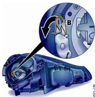
Halogen headlights
