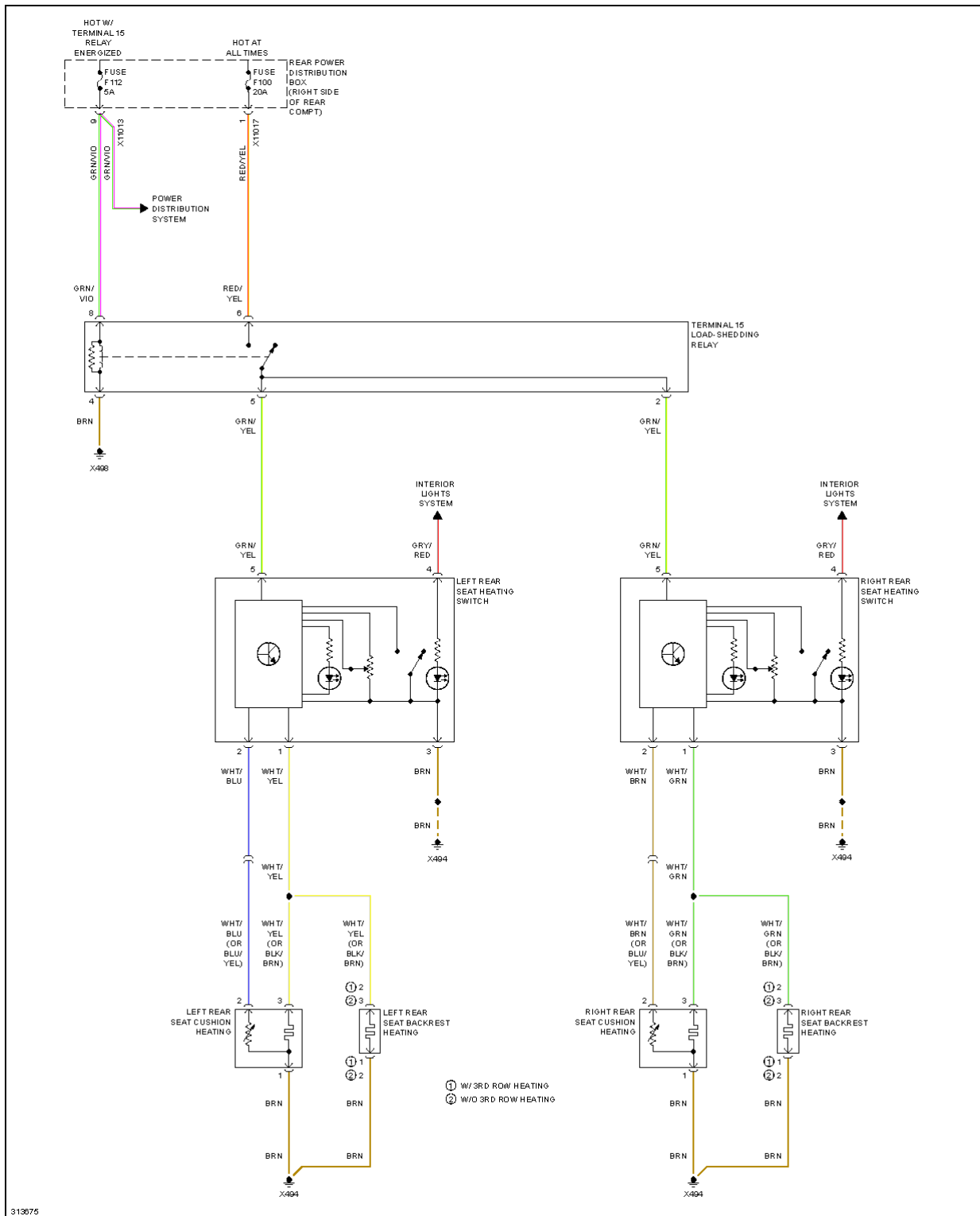
Fig. 98: Rear Heated Seats Circuit, W/O Rear A/C
