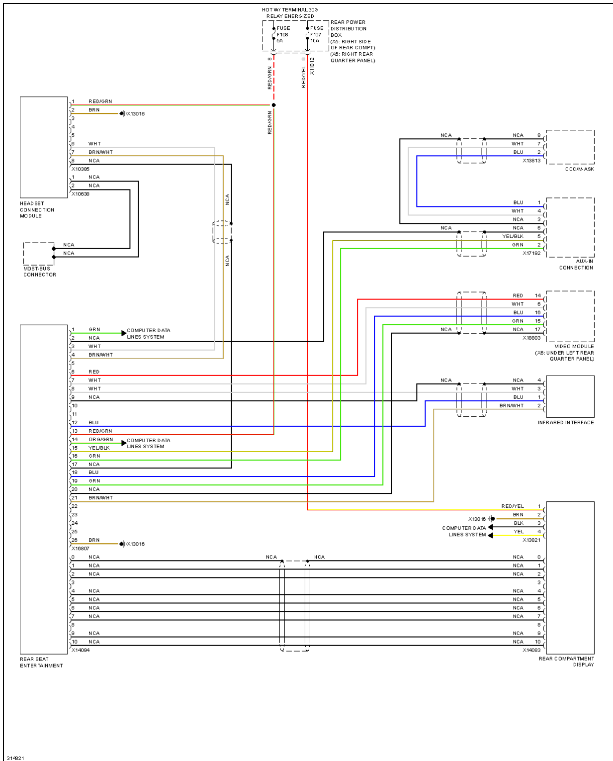
Fig. 115: Rear Seat Entertainment Circuit
