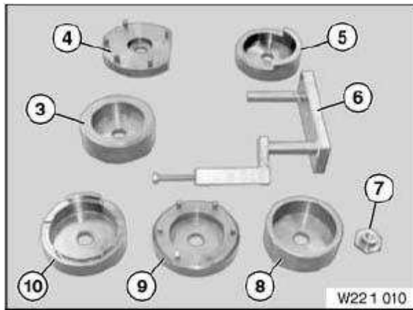
Fig. 1: Identify Special Tool (22 1 010)
