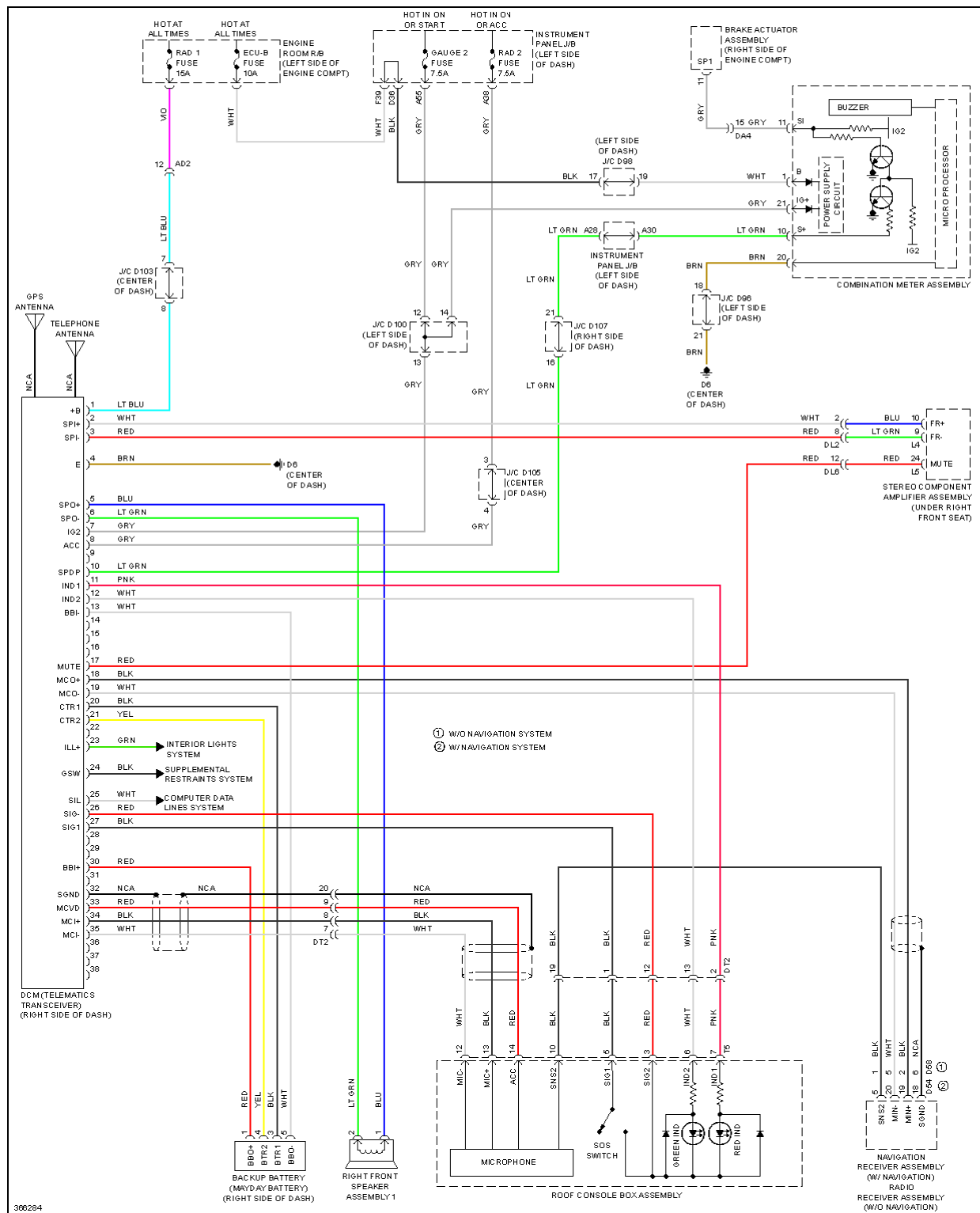
Fig. 68: Telematics Circuit
