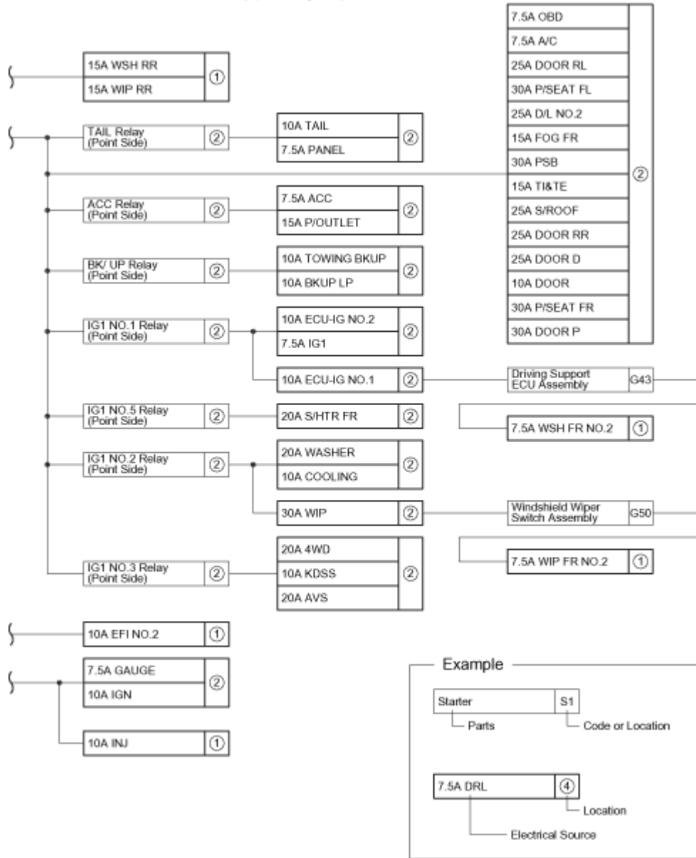
Fig. 2: Current Flow Chart (2 Of 2)
