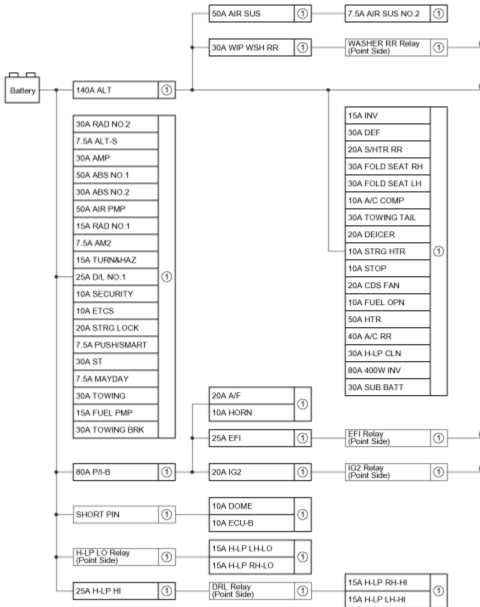
Fig. 1: Current Flow Chart (1 Of 2)
