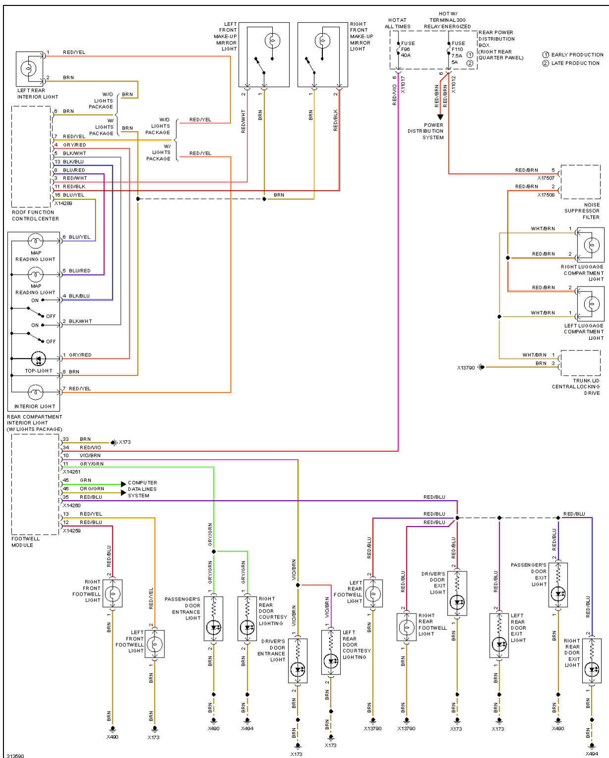
Fig. 57: Courtesy Lamps Circuit
