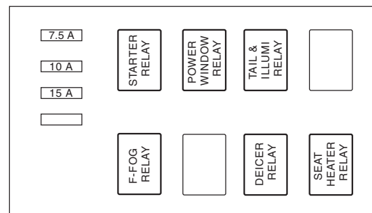
RELAY BLOCK
