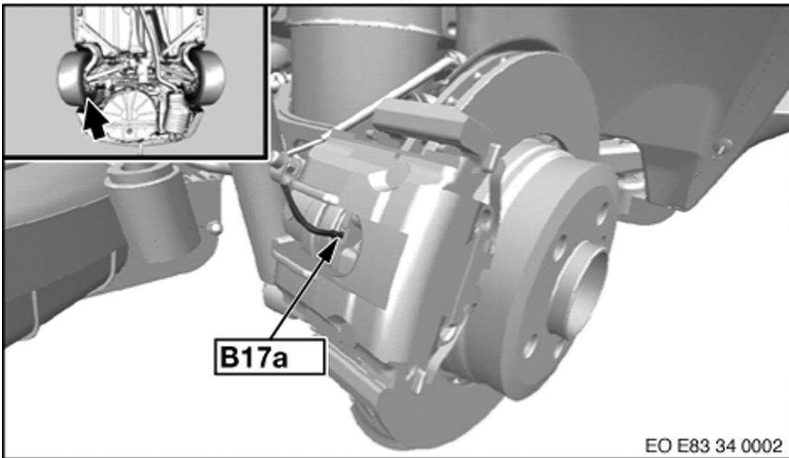
Fig. 28: Right Rear Wheel
