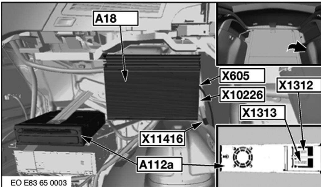
Fig. 49: Left Side Of Rear Compartment
