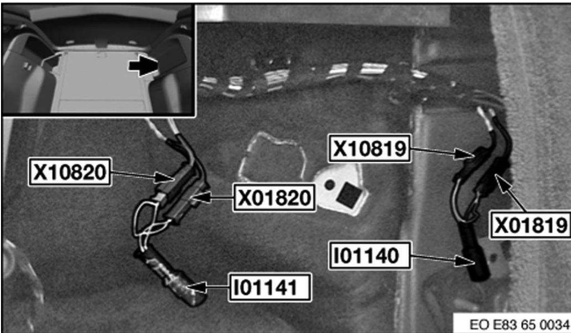
Fig. 99: Left Side Of Rear Compartment
