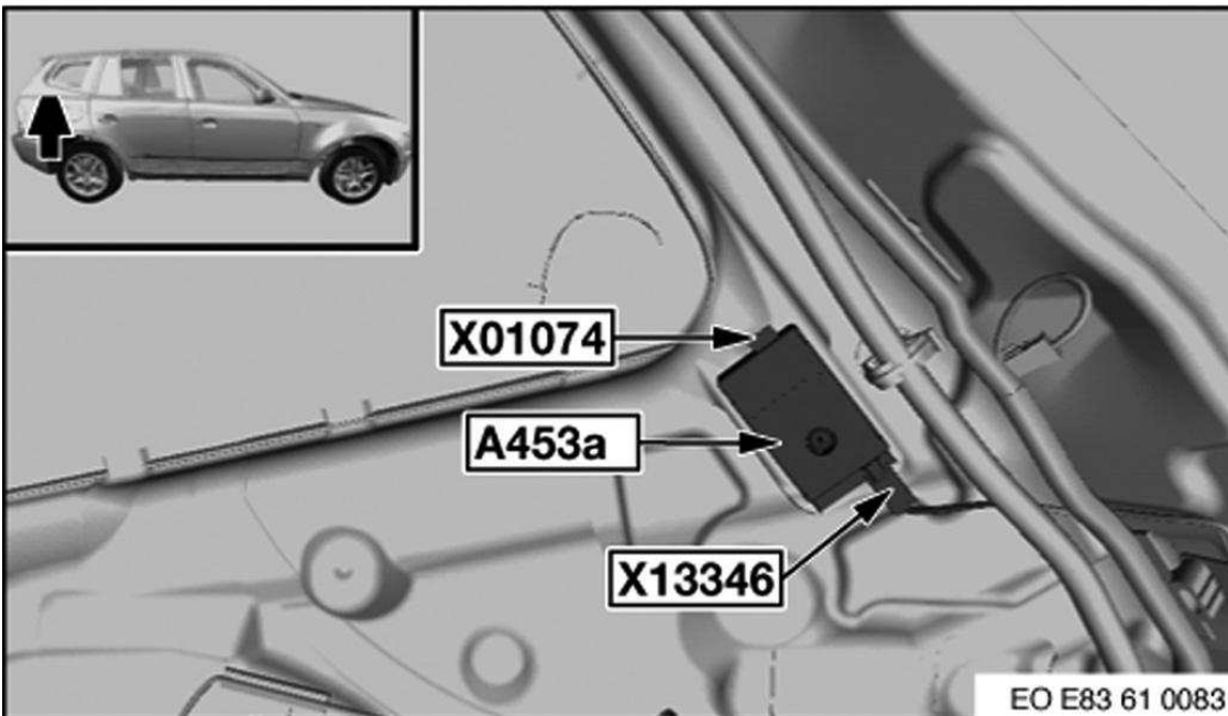
Fig. 67: Right Side Of Rear Compartment
