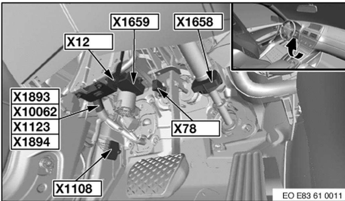
Fig. 6: Left Kick Panel
