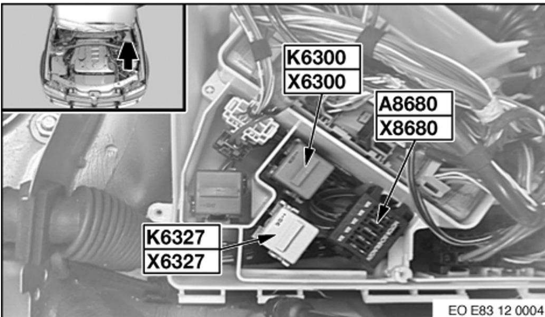
Fig. 33: Left Rear Of Engine Compartment
