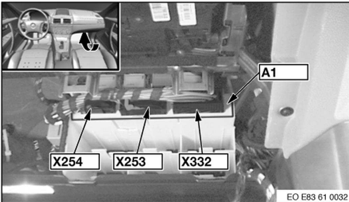
Fig. 18: Right Side Of Dash
