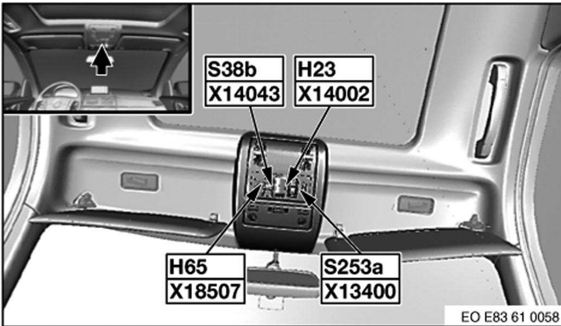
Fig. 80: Overhead Console
