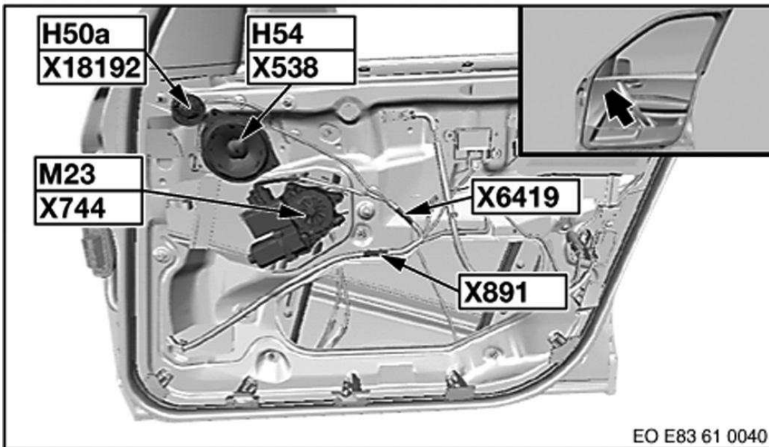
Fig. 62: Front Passenger's Door
