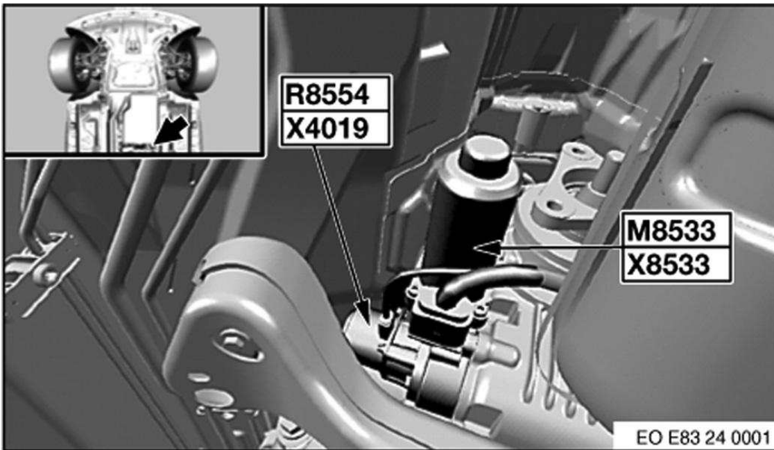
Fig. 112: Under Vehicle
