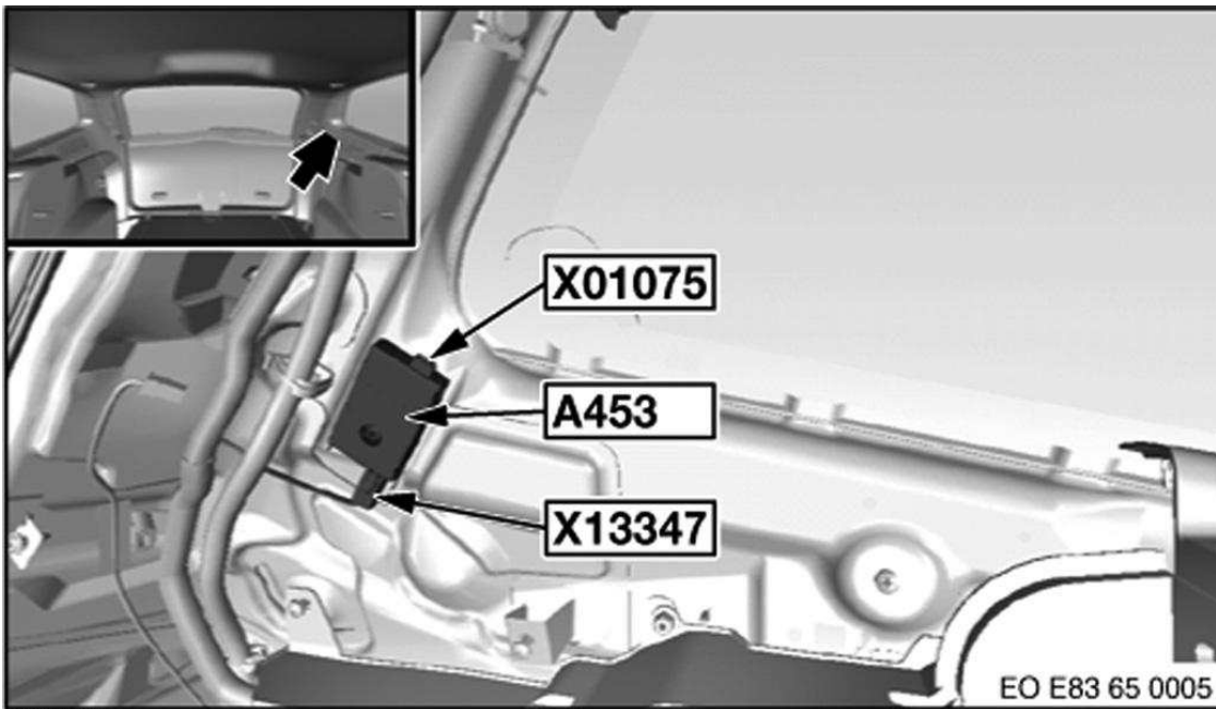
Fig. 66: Bottom Of Left "C" Pillar
