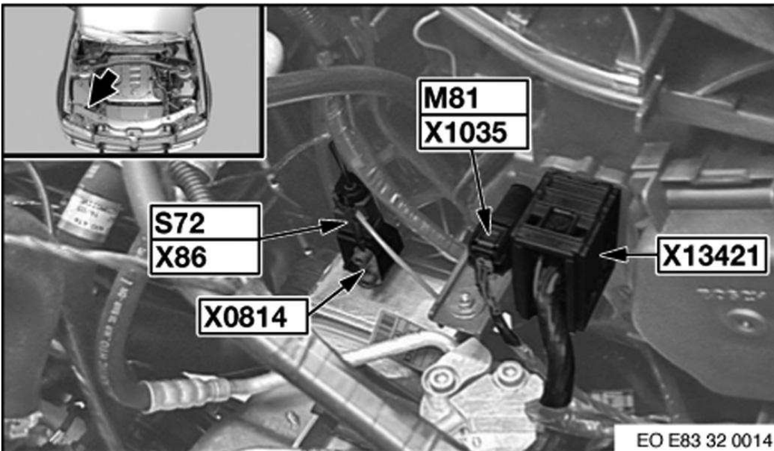
Fig. 95: Right Side Of Engine Compartment
