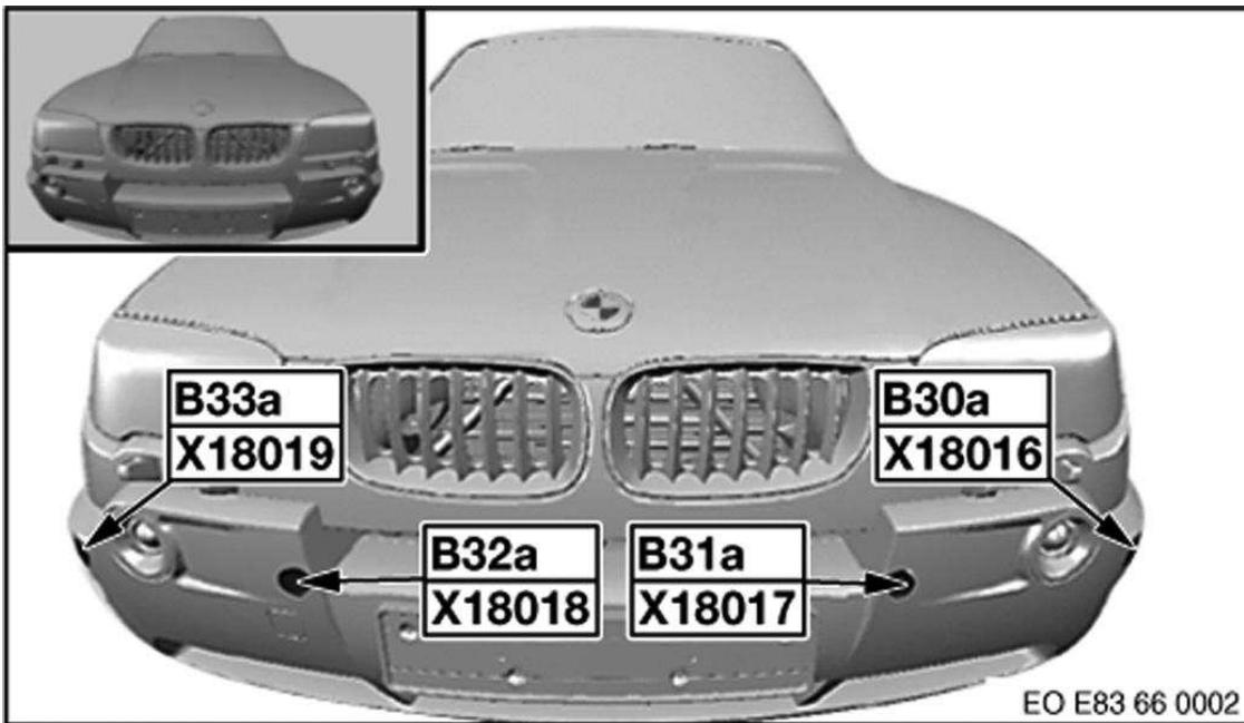
Fig. 74: Front Bumper
