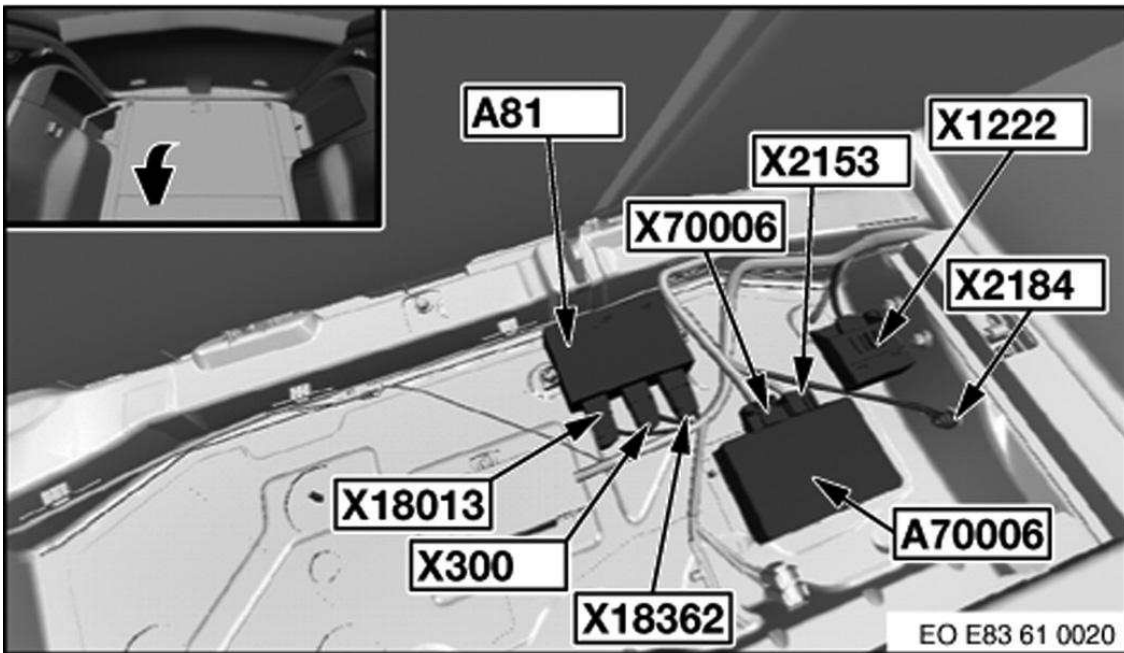
Fig. 54: Rear Compartment
