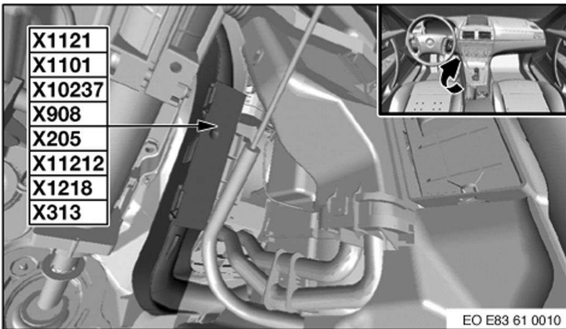
Fig. 8: Center Of Dash
