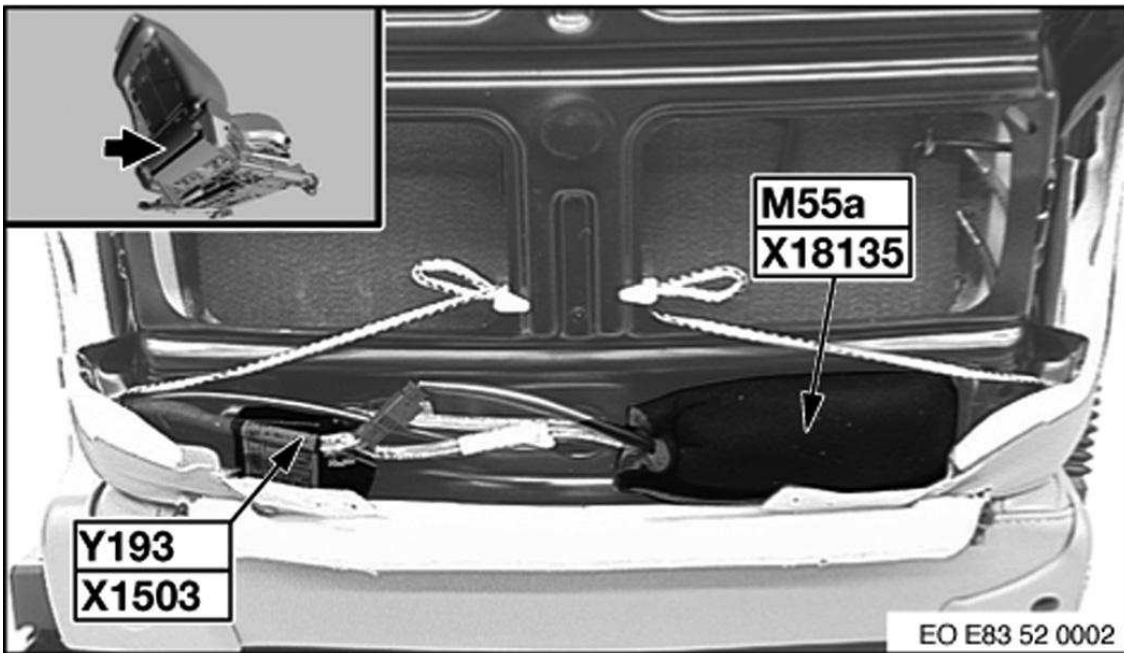
Fig. 108: Under Driver's Seat Courtesy of BMW OF NORTH AMERICA, INC.
