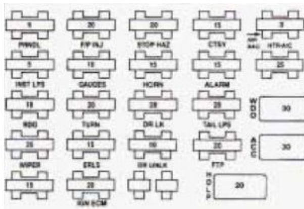
Oldsmobile Achieva – fuse box
