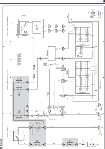
CELICA (EWD503E)
