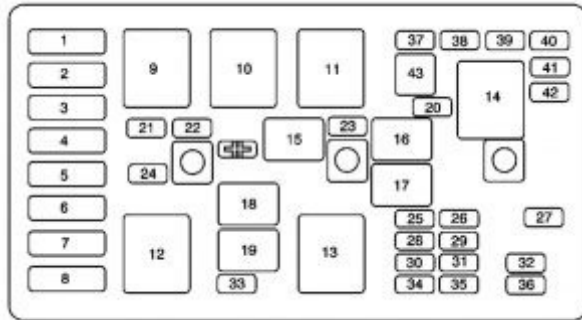
Buick regal mk4 – fuse box – engine
