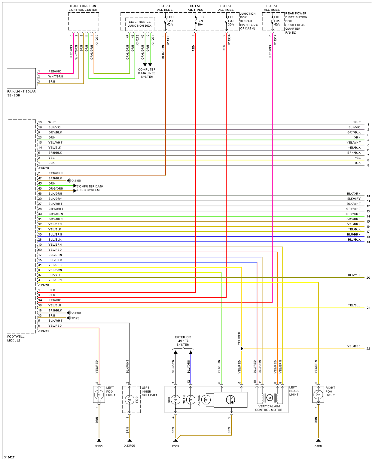
Fig. 52: Headlamps Circuit, W/ Xenon Lamps (1 of 2)
