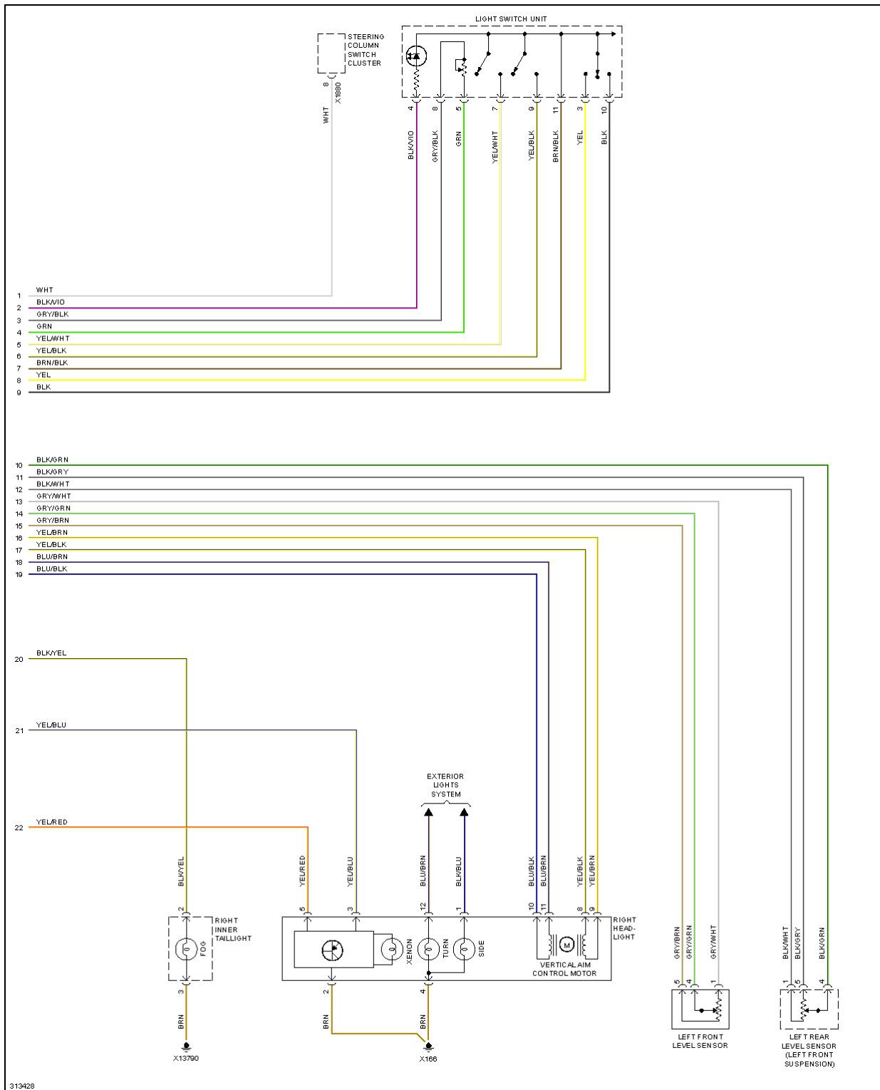
Fig. 53: Headlamps Circuit, W/ Xenon Lamps (2 of 2)
