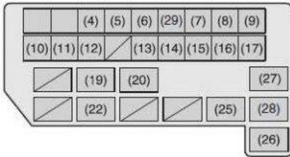
Suzuki SX4 – fuse box diagram – engine compartment (diesel)
