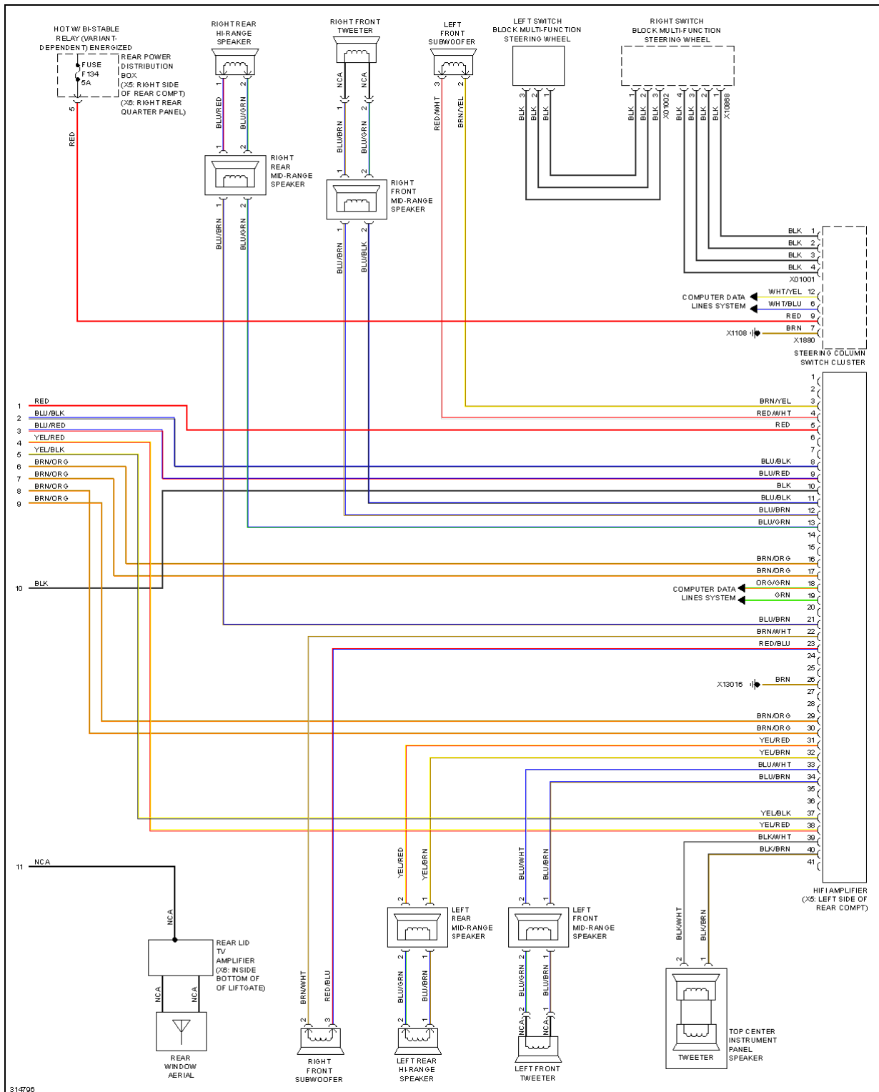
Fig. 77: Navigation Circuit, W/O CIC & W/ HiFi Radio (3 of 3)
