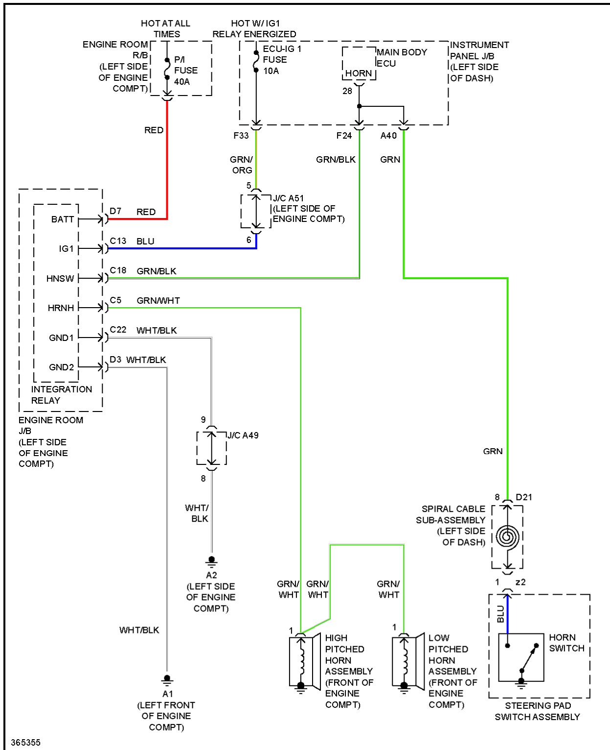
Fig. 50: Horn Circuit
