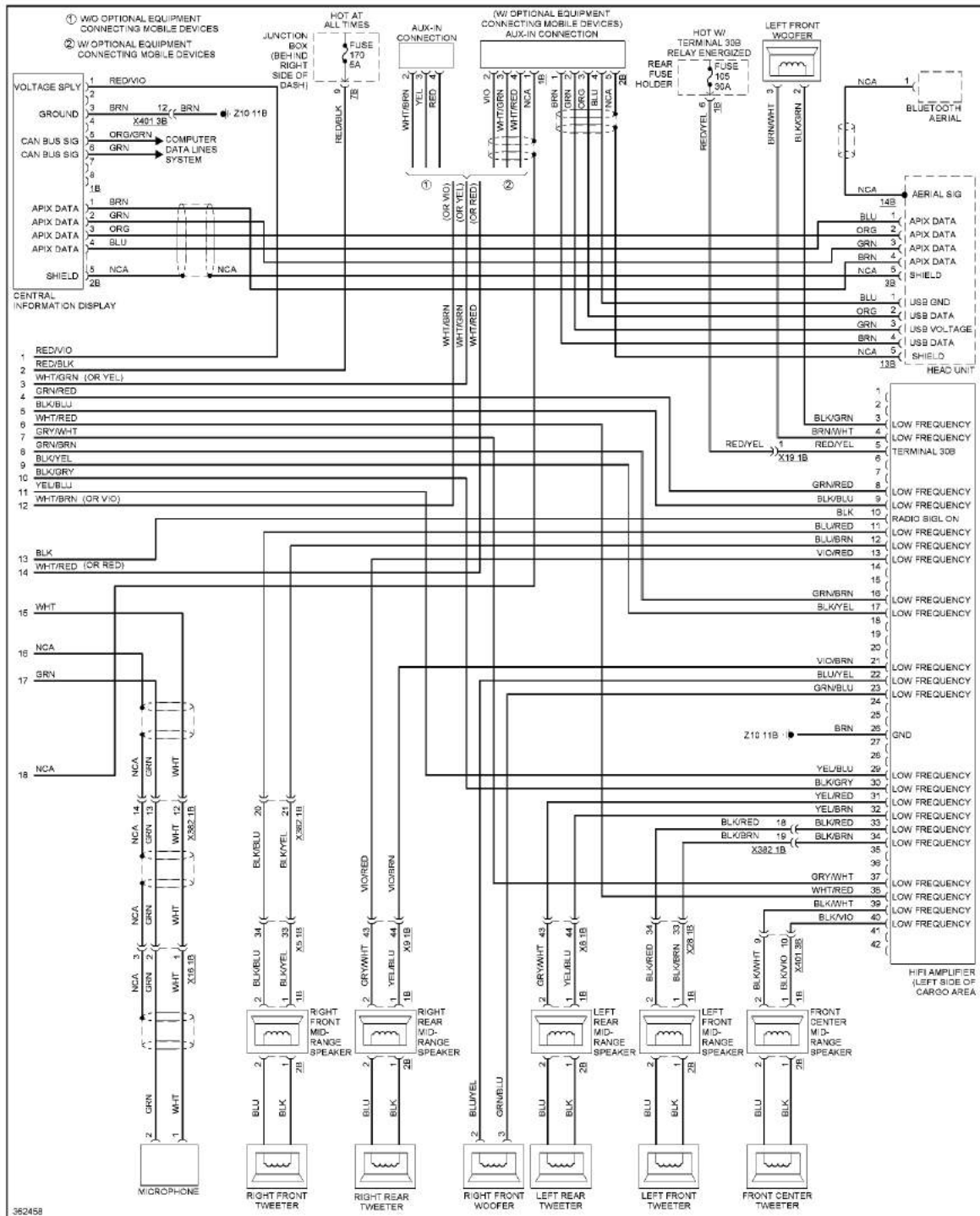
Fig. 51: Navigation Circuit, W/ HiFi Radio (2 of 2)
