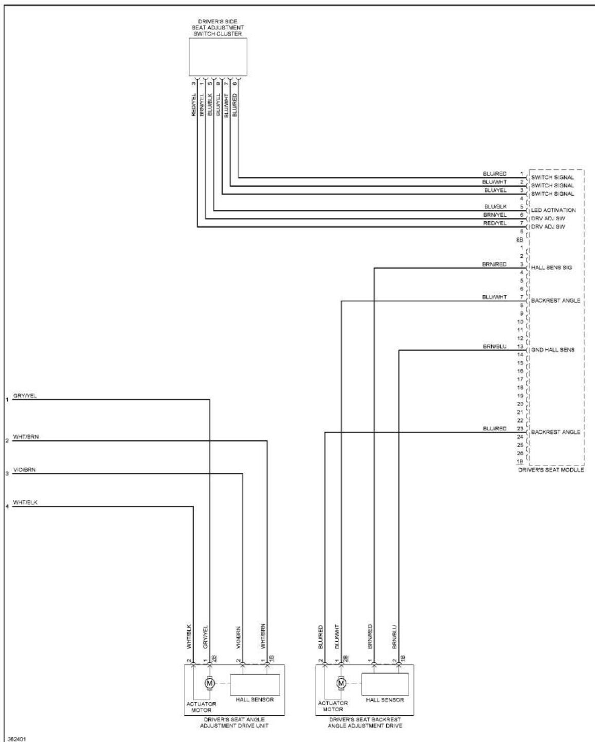
Fig. 49: Memory Systems Circuit (2 of 2)
