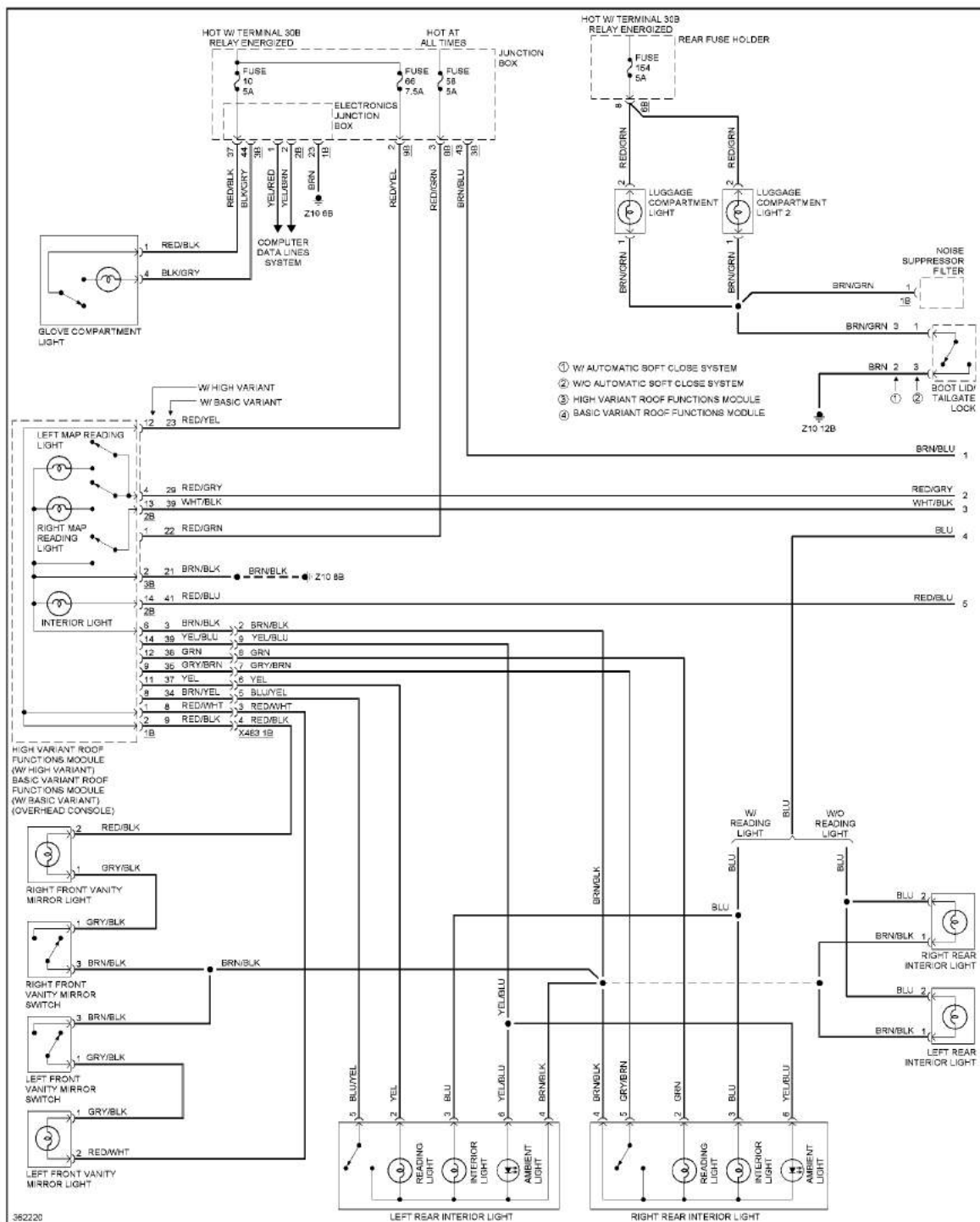
Fig. 44: Courtesy Lamps Circuit (1 of 2)
