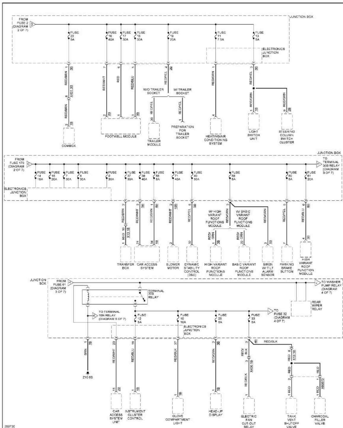
Fig. 58: Power Distribution Circuit (3 of 7)
