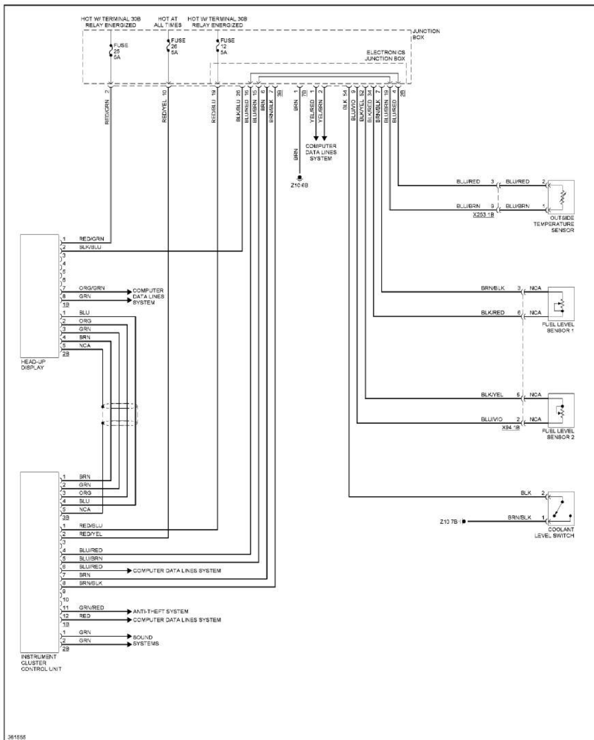
Fig. 43: Instrument Cluster Circuit
