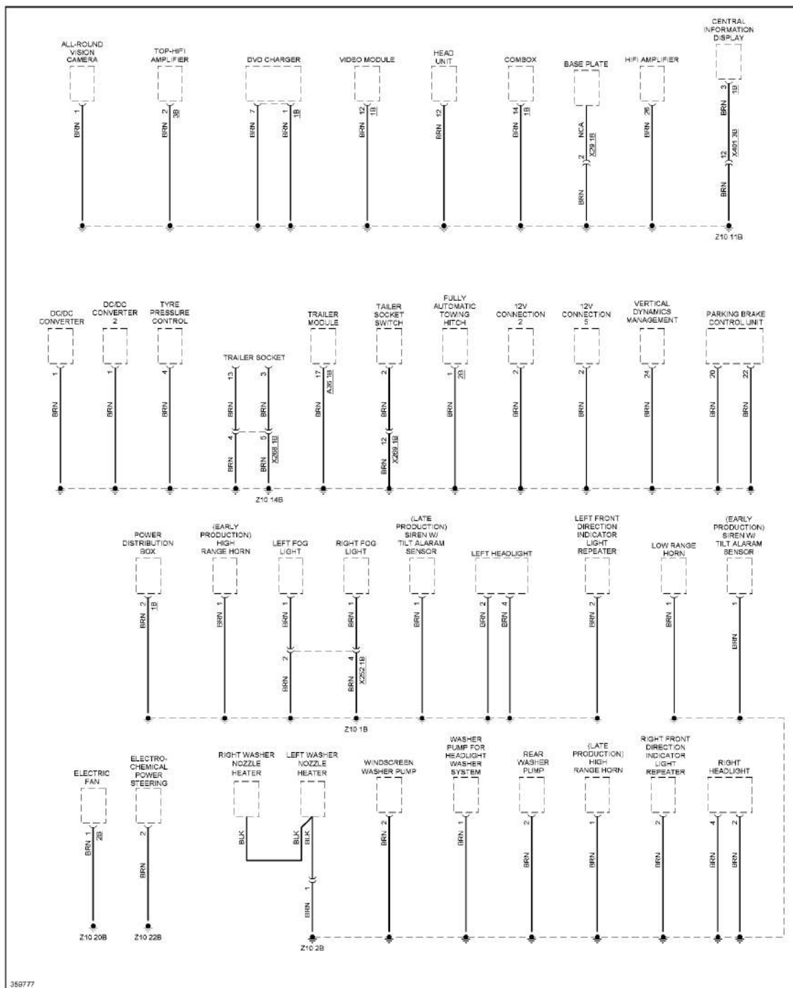
Fig. 38: Ground Distribution Circuit (3 of 4)
