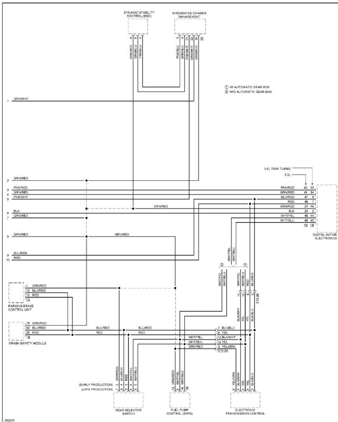
Fig. 13: Computer Data Lines Circuit (3 of 3)
