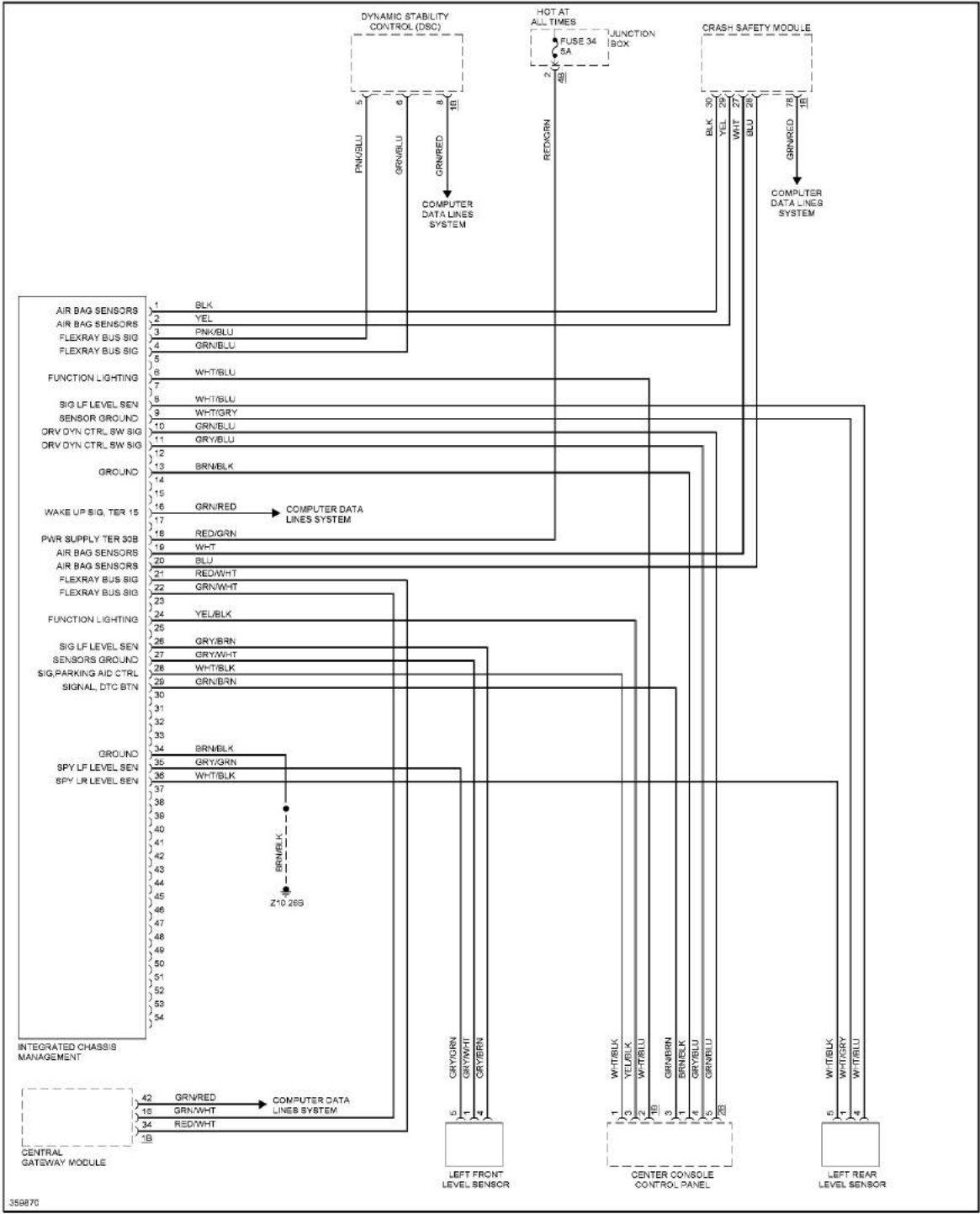
Fig. 20: Air Suspension Circuit
