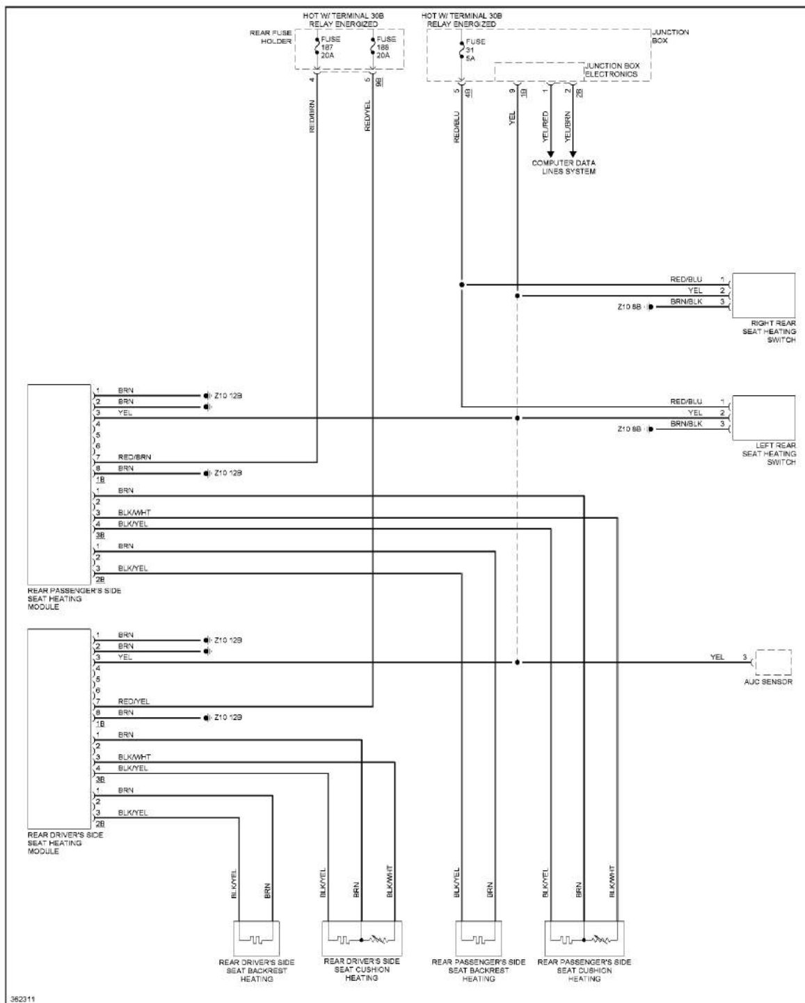
Fig. 73: Rear Heated Seats Circuit
