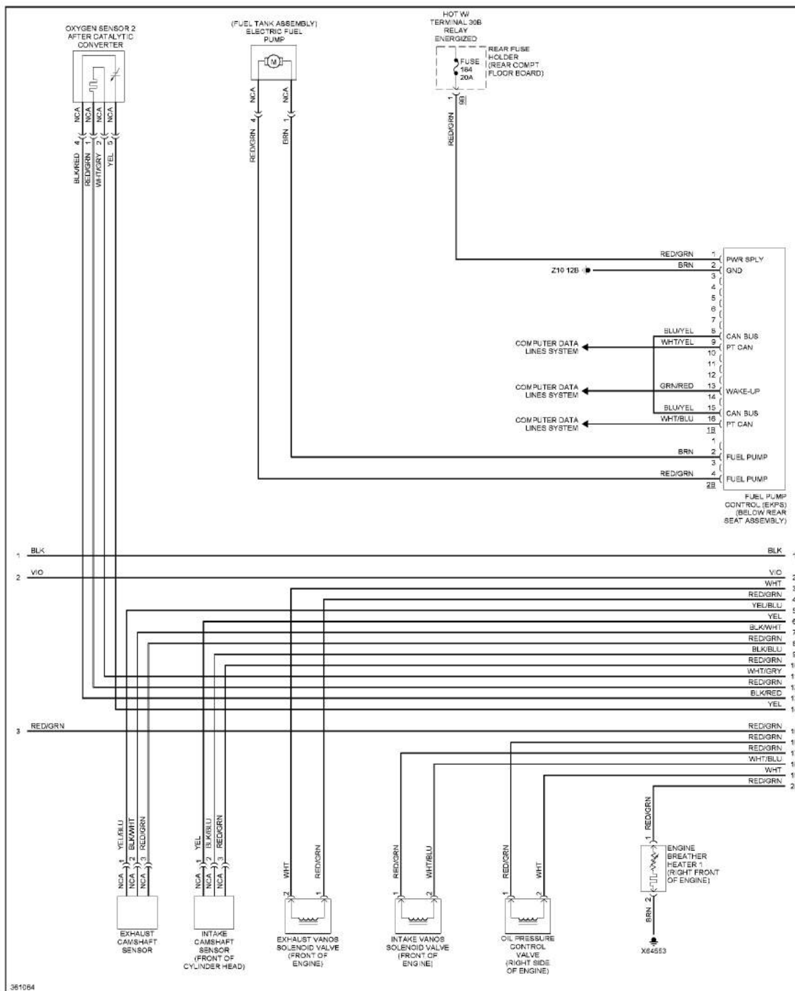
Fig. 23: 3.0L Engine Performance Circuit (2 of 5)
