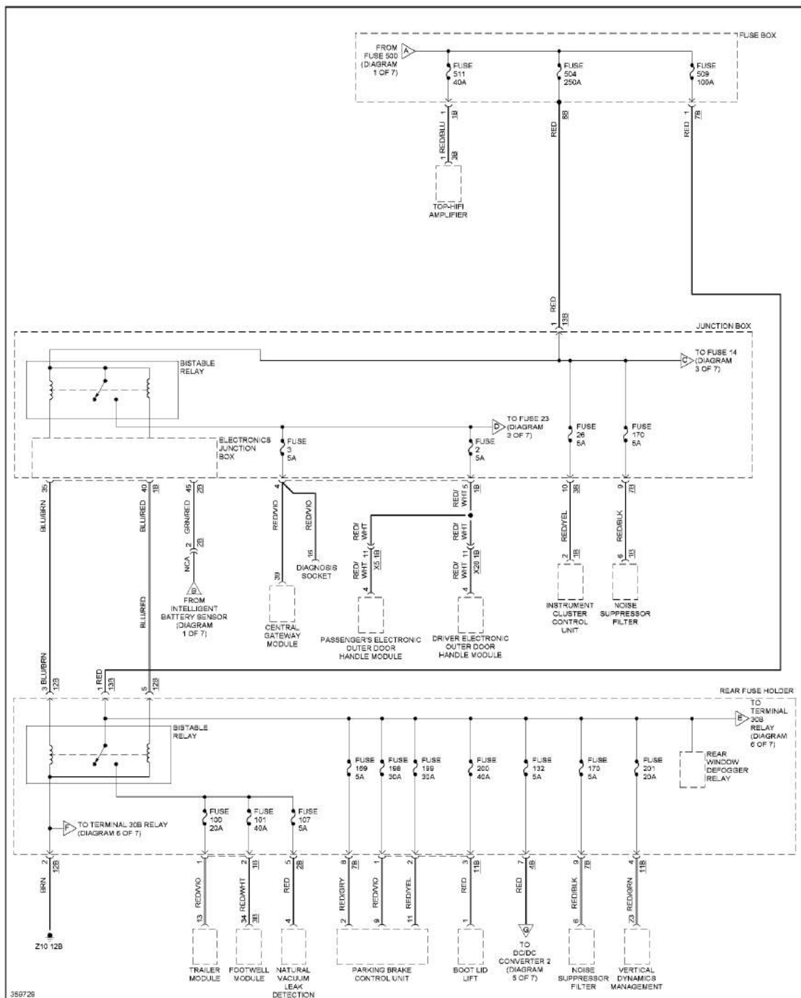
Fig. 57: Power Distribution Circuit (2 of 7)
