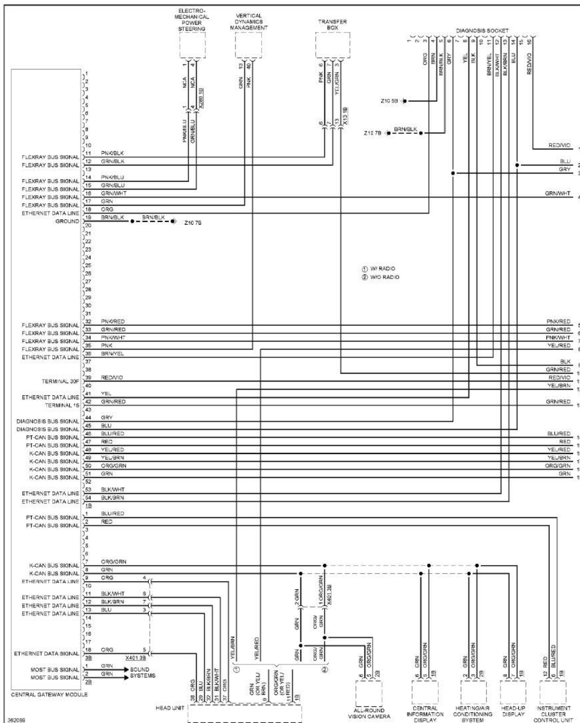
Fig. 11: Computer Data Lines Circuit (1 of 3)
