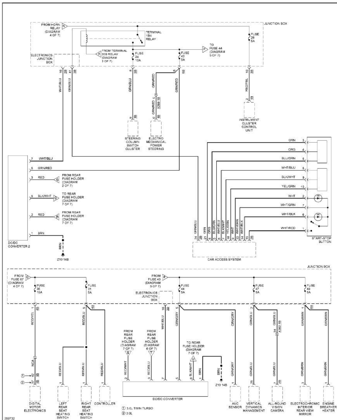
Fig. 60: Power Distribution Circuit (5 of 7)
