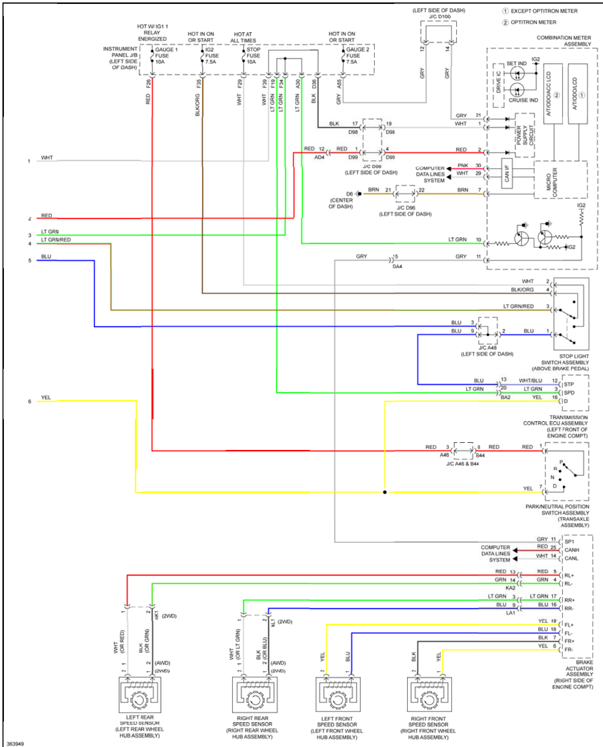
Fig. 22: 3.5L, Cruise Control Circuit (2 of 2)
