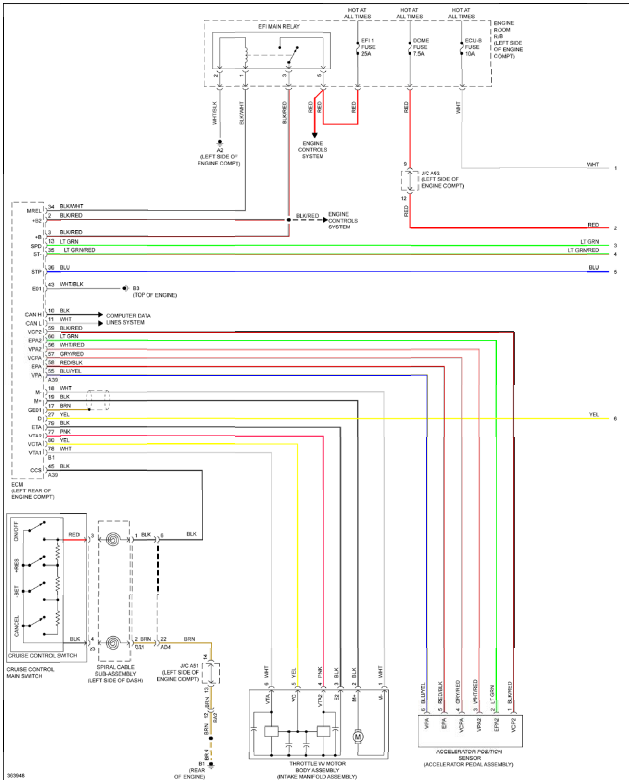
Fig. 21: 3.5L, Cruise Control Circuit (1 of 2)
