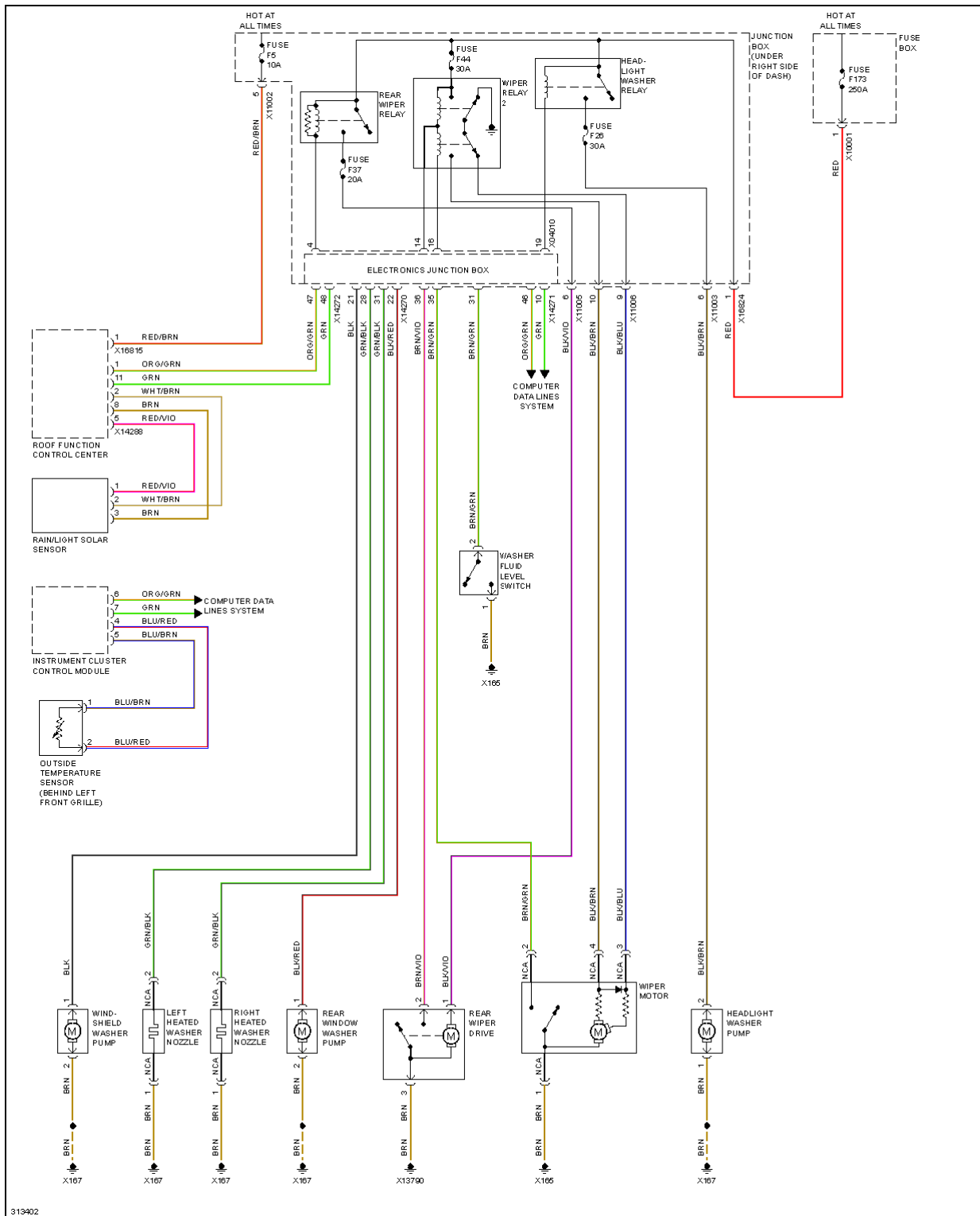
Fig. 129: Wiper/Washer Circuit
