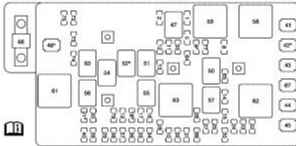
GMC Canyon mk1 – fuse box – engine
