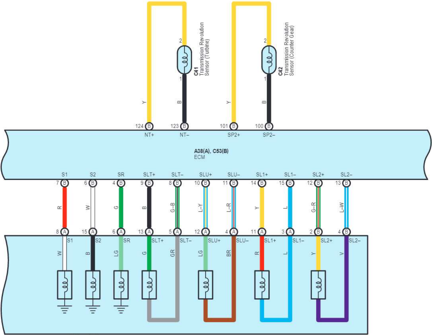
C39(A), C40(B) Electronically Controlled Transmission Solenoid
