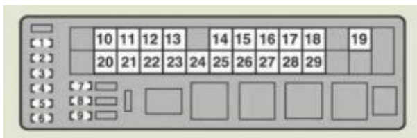
Lexus IS250 – fuse box – engine compartment (type A) – left-hand drive vehicle
