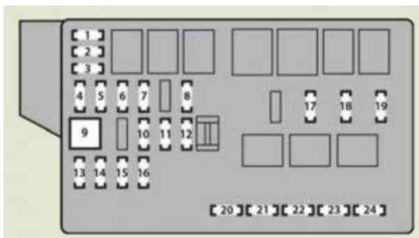
Lexus IS250 – fuse box –
