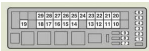
Lexus IS250 – fuse box – engine compartment (type A) – right-hand drive vehicle
