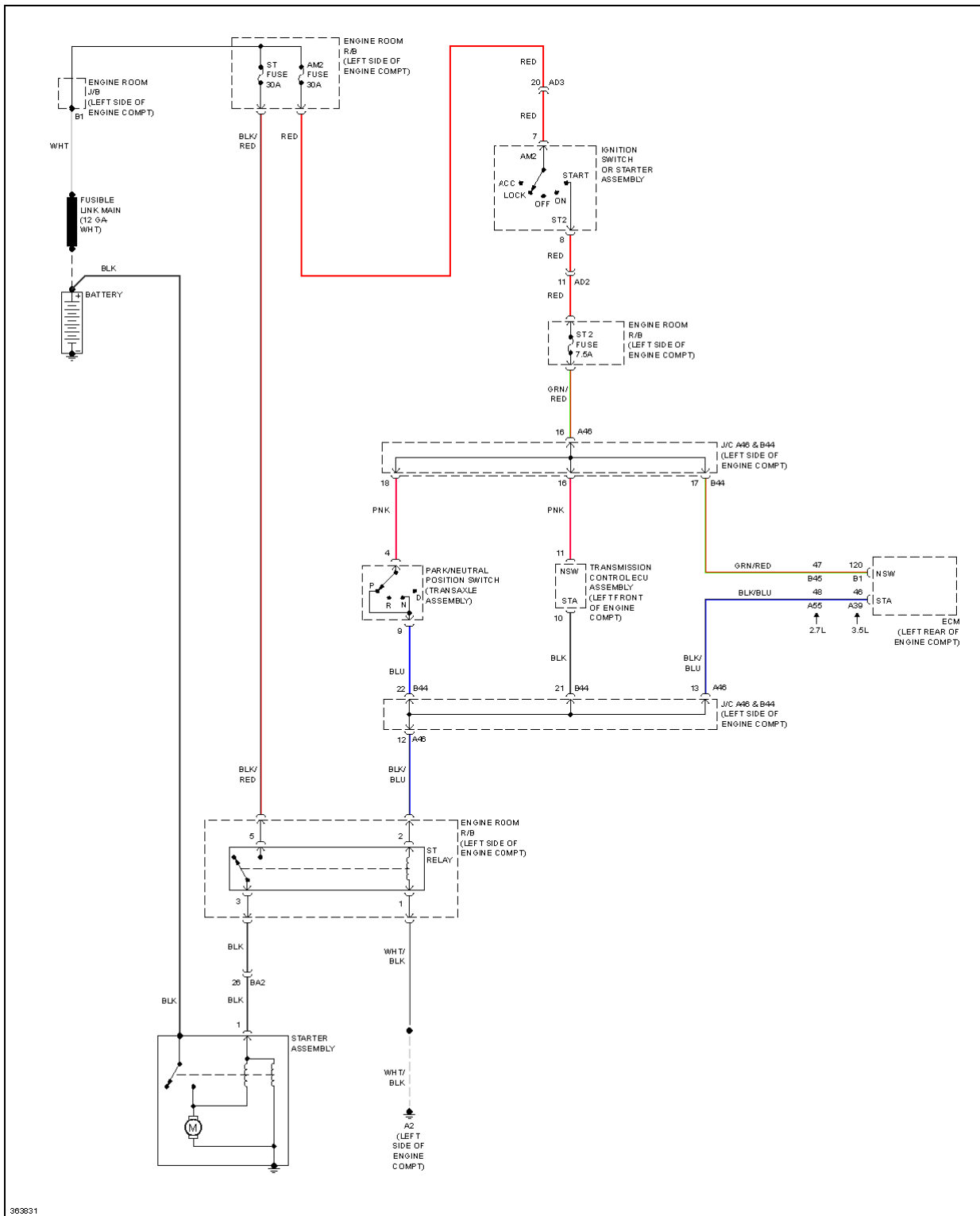
Fig. 107: Starting Circuit, W/O Smart Key System
