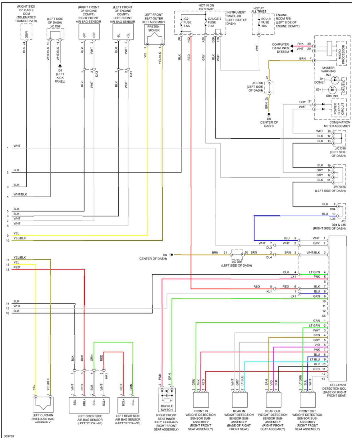
Fig. 110: Supplemental Restraint Circuit (2 of 2)
