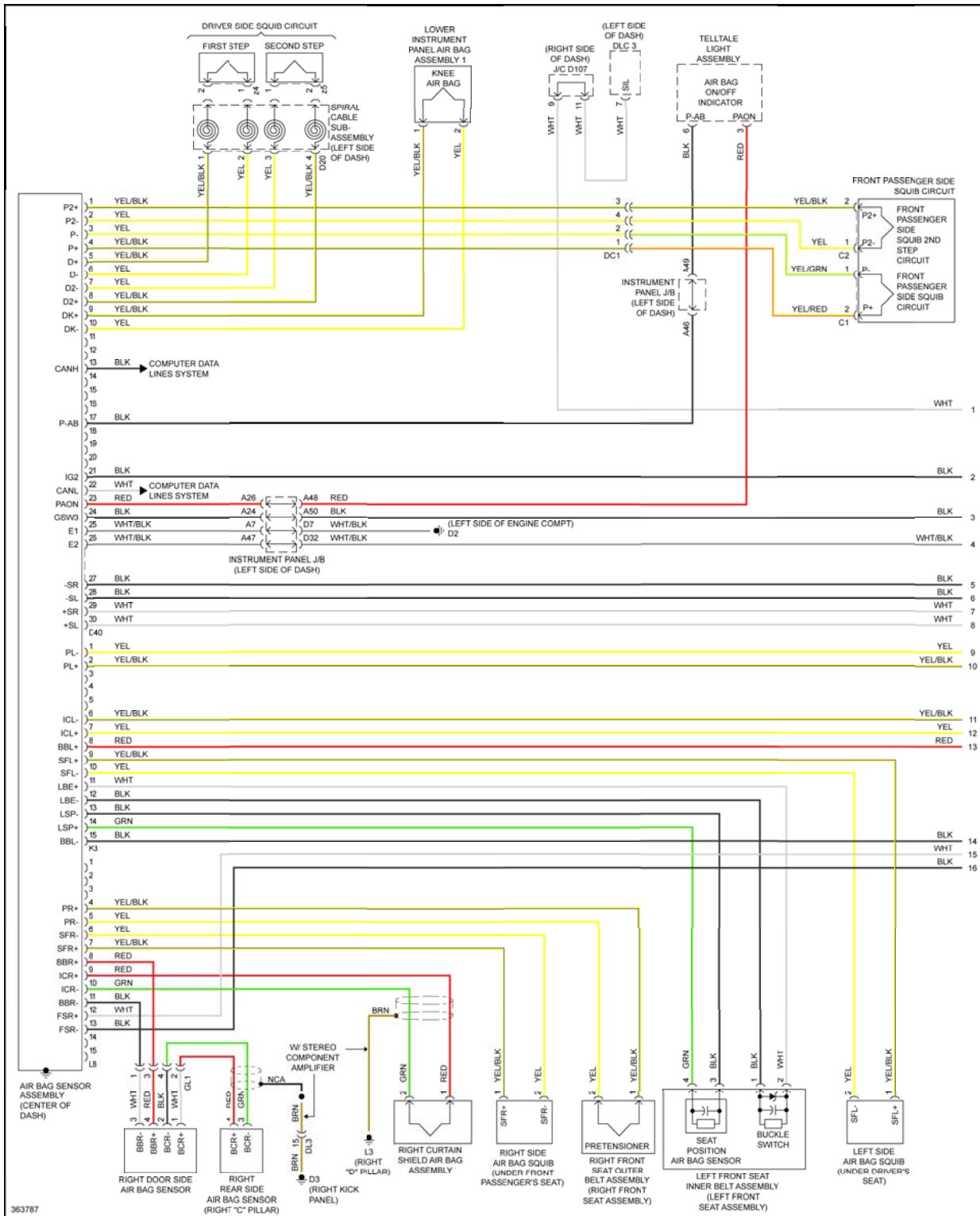
Fig. 109: Supplemental Restraint Circuit (1 of 2)
