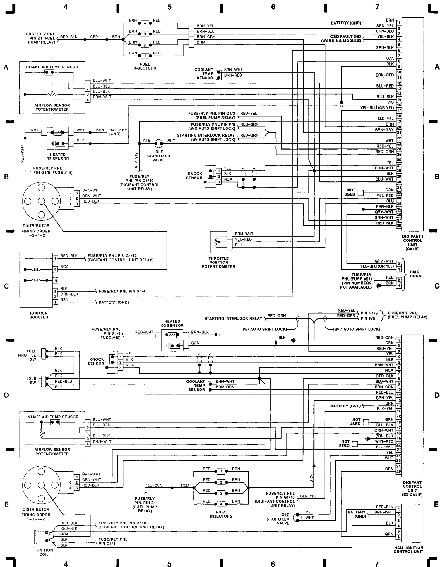
Fig. 2: Digifant Control Unit (Grid 4-7) 1992 Volkswagen Jetta GL
