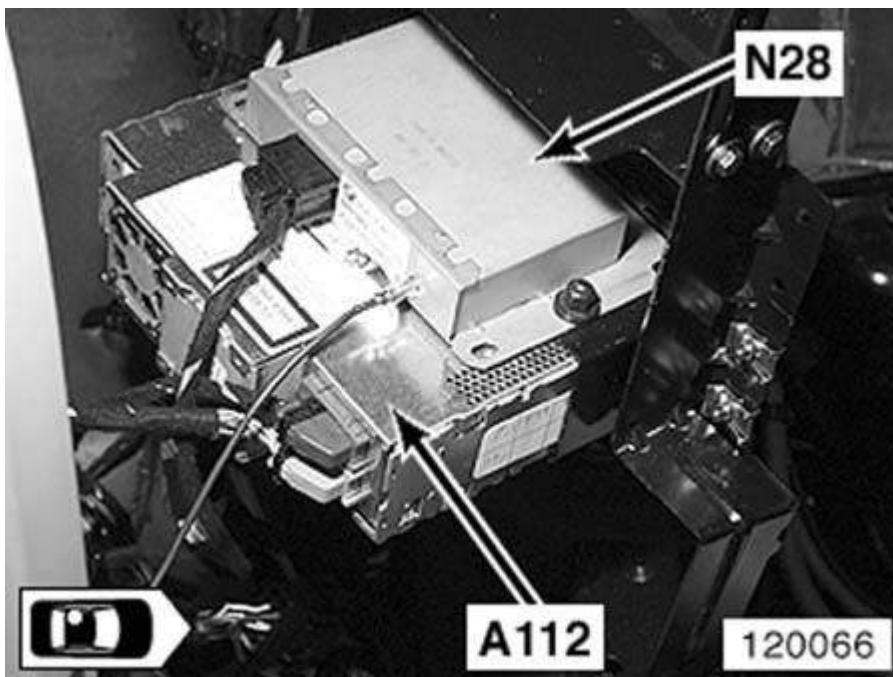
Fig. 23: Left Rear Of Passenger Compartment
