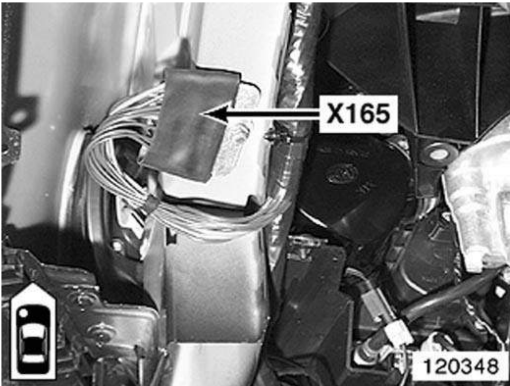
Fig. 4: Left Front Wheelwell
