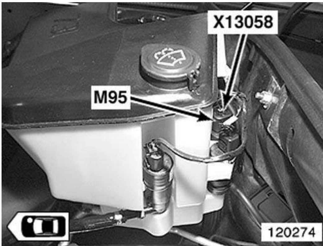
Fig. 50: Washer Reservoir
