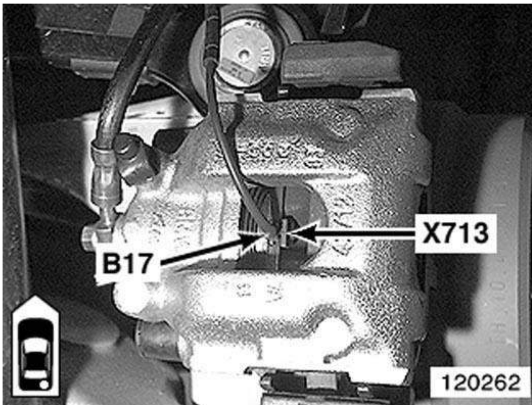
Fig. 32: Right Rear Brake Caliper
