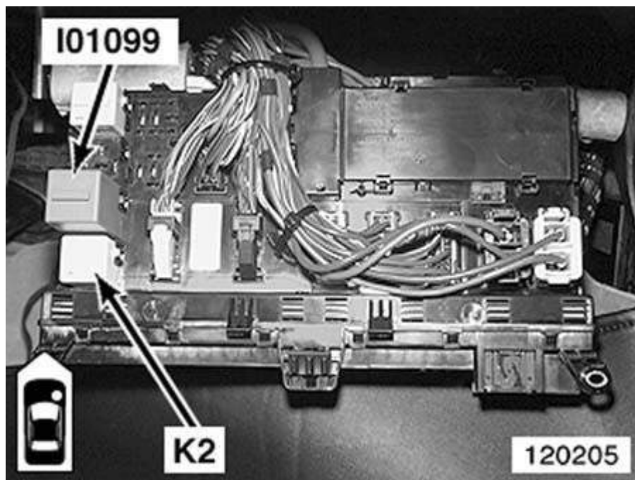
Fig. 44: Behind Glove Box Courtesy of BMW OF NORTH AMERICA, INC.
