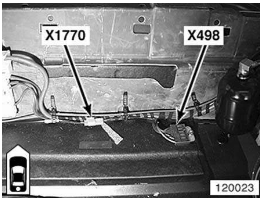
Fig. 17: Front Center Of Luggage Compartment Courtesy of BMW OF NORTH AMERICA, INC.
