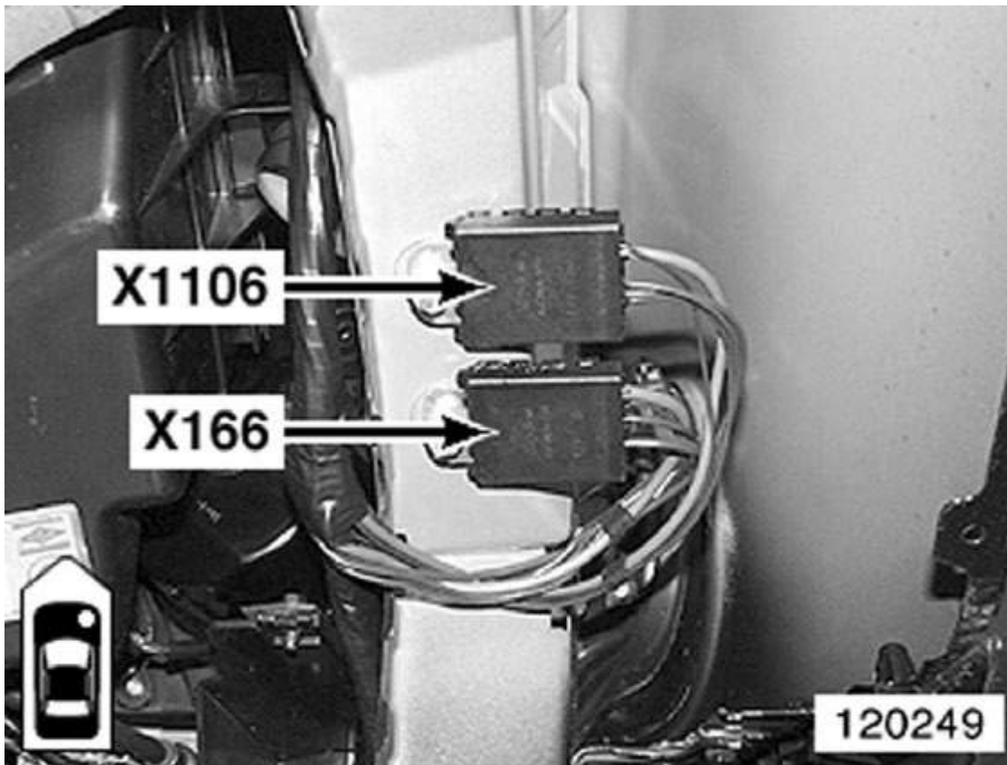
Fig. 5: Right Front Wheelwell
