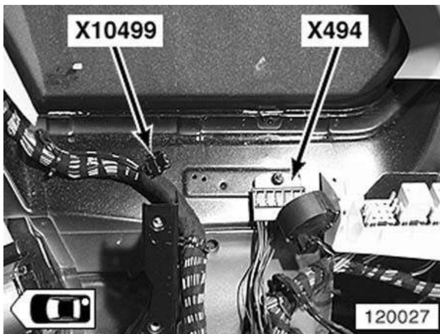
Fig. 16: Right Rear Of Passenger Compartment Courtesy of BMW OF NORTH AMERICA, INC.
