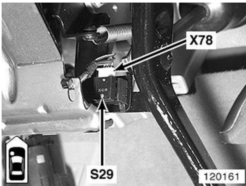
Fig. 54: Under Left Side Of Dash
