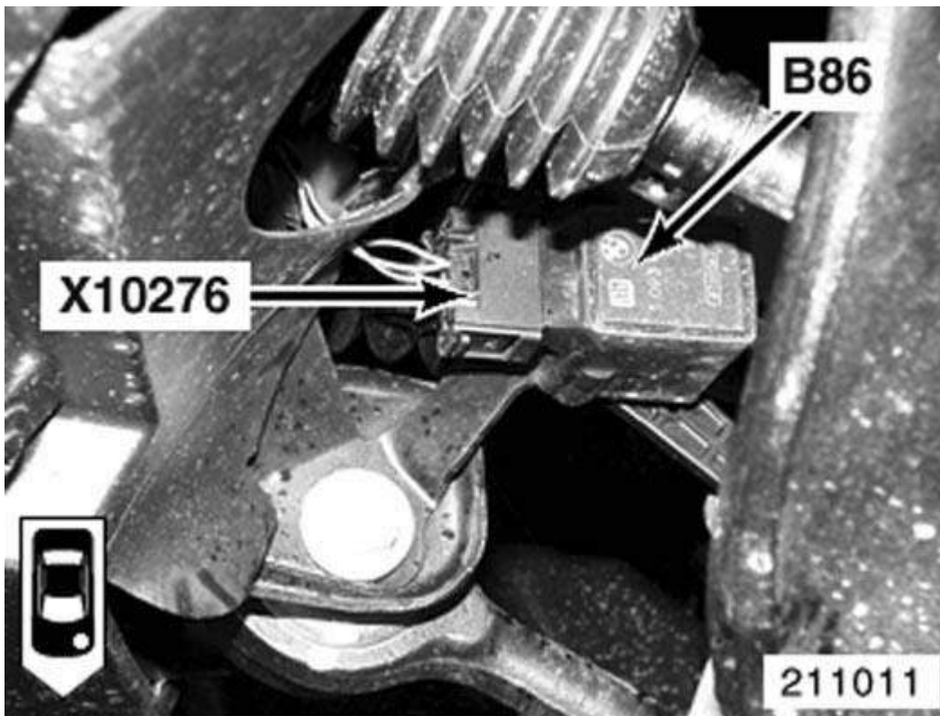
Fig. 36: Left Front Control Arm
