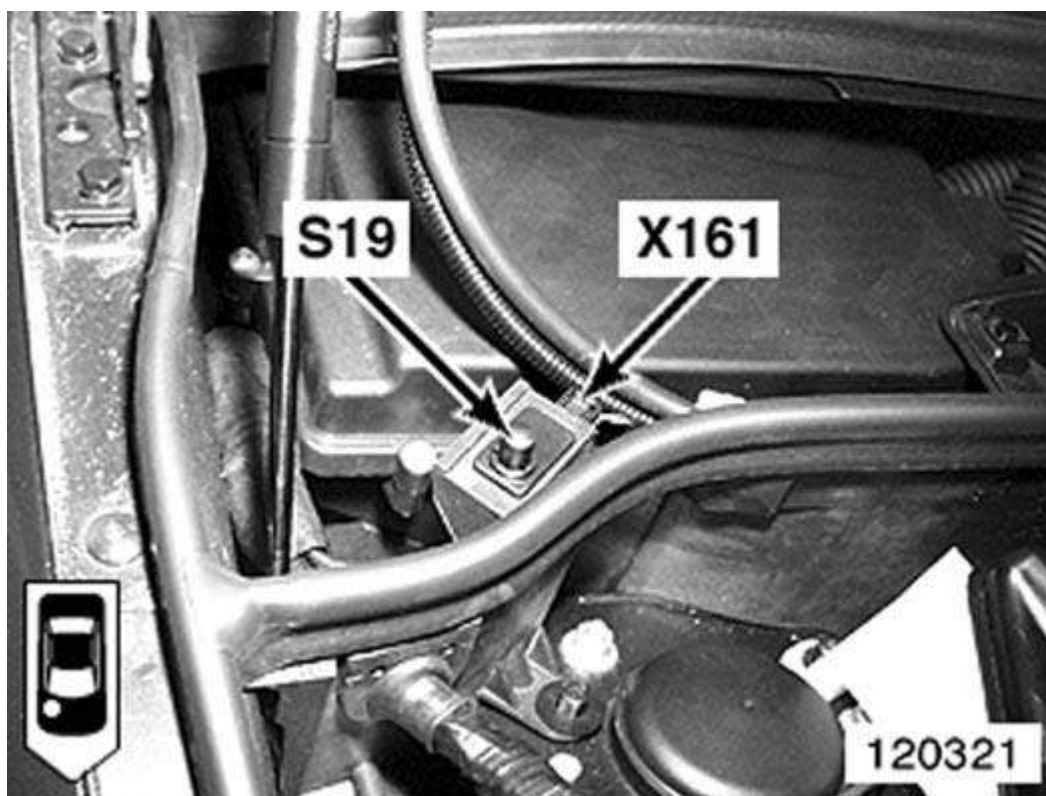
Fig. 53: Right Rear Of Engine Compartment Courtesy of BMW OF NORTH AMERICA, INC.
