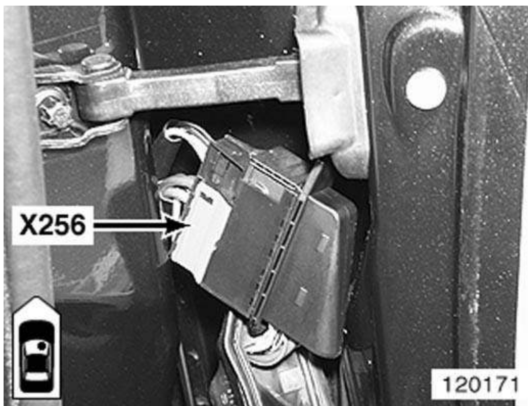
Fig. 12: Passenger's Door
