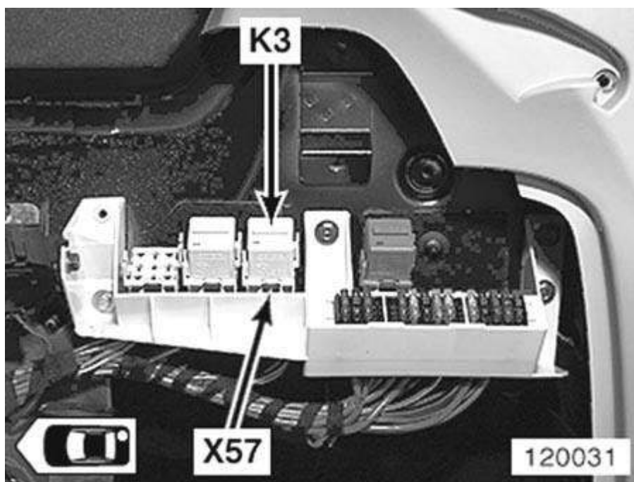
Fig. 45: Right Rear Of Luggage Compartment Courtesy of BMW OF NORTH AMERICA, INC.
