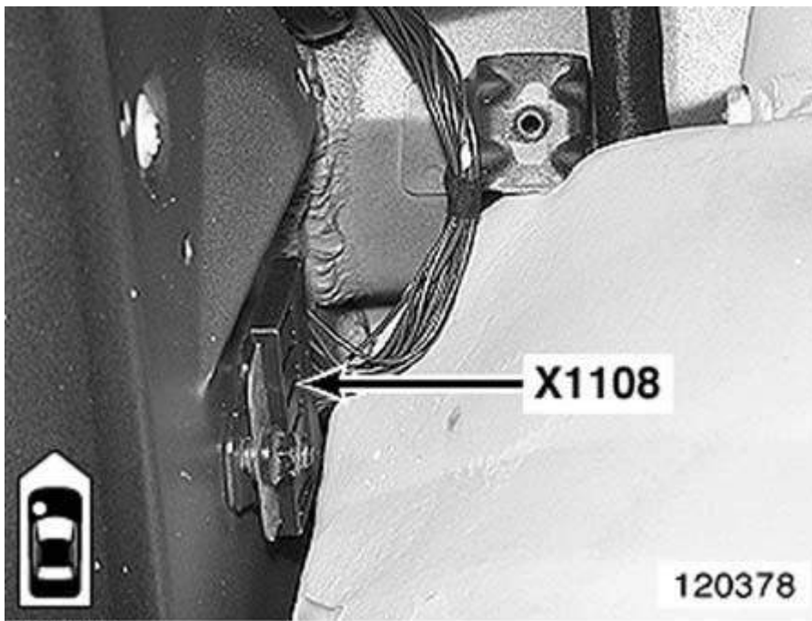
Fig. 6: Left Kick Panel
