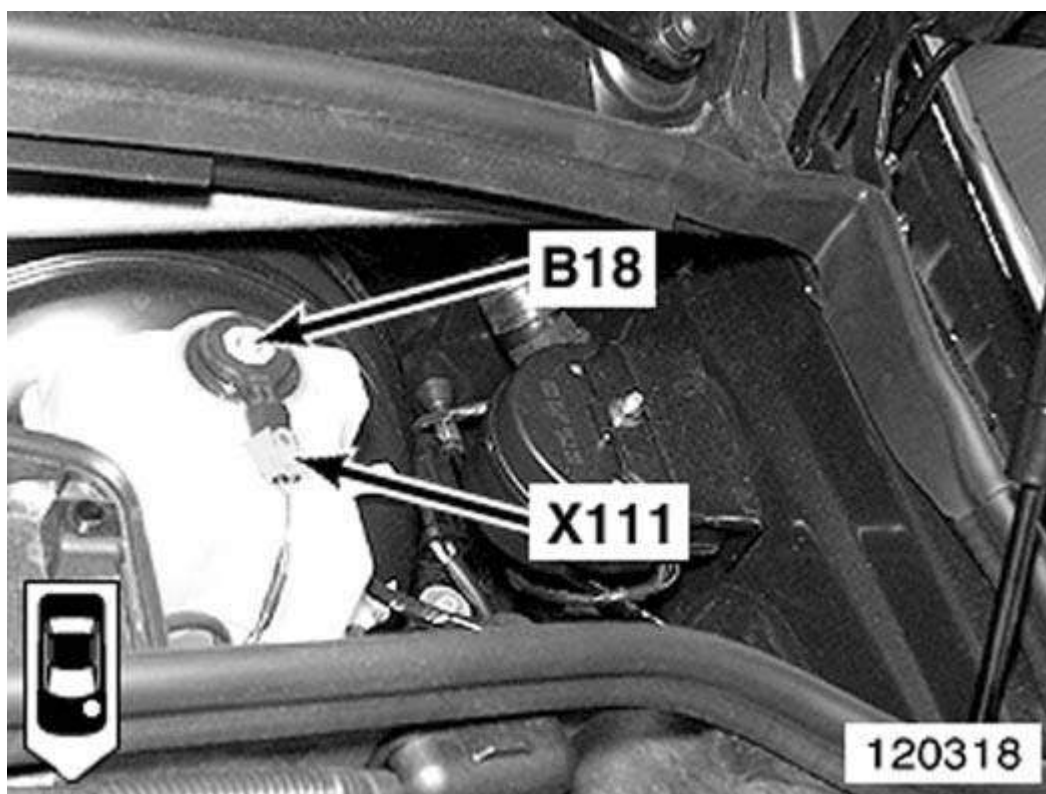
Fig. 33: Left Rear Of Engine Compartment Courtesy of BMW OF NORTH AMERICA, INC.
