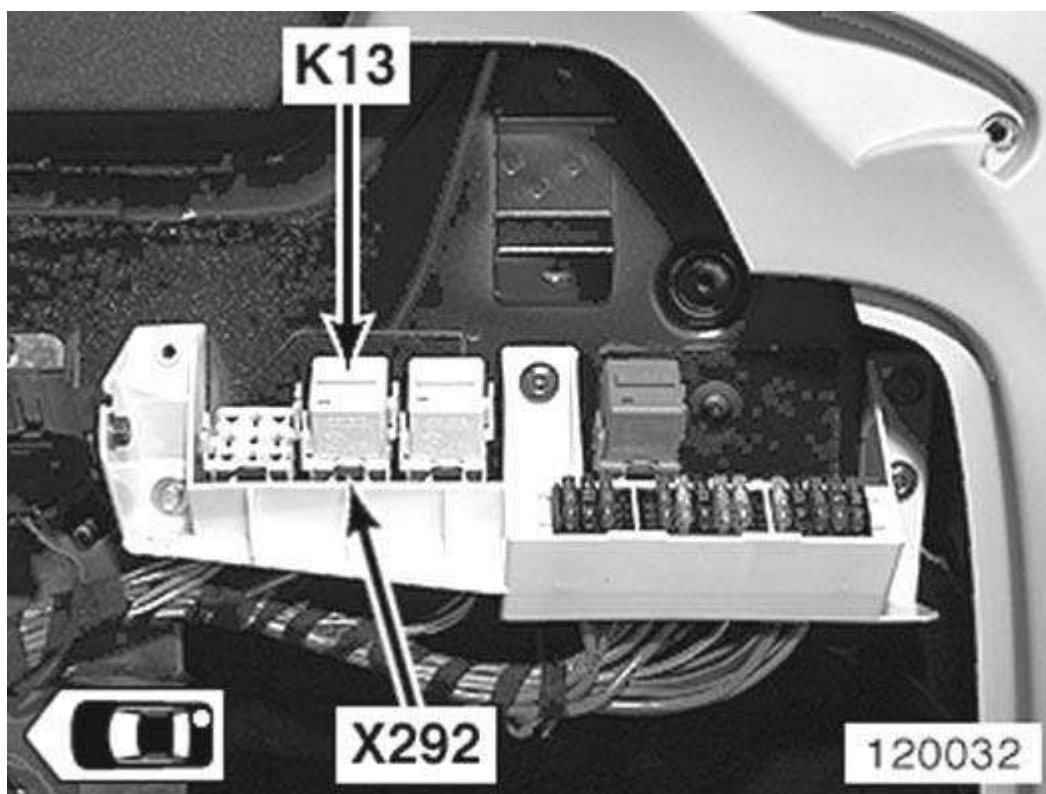
Fig. 46: Right Rear Of Luggage Compartment
