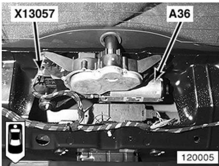
Fig. 21: Tailgate
