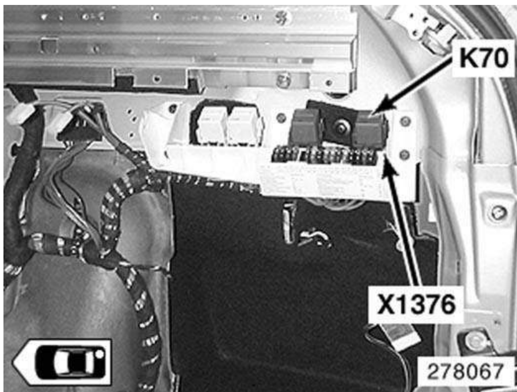
Fig. 47: Right Rear Of Luggage Compartment Courtesy of BMW OF NORTH AMERICA, INC.
