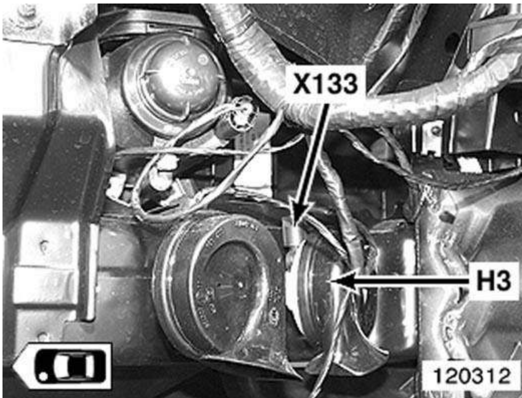
Fig. 40: Left Front Wheelwell
