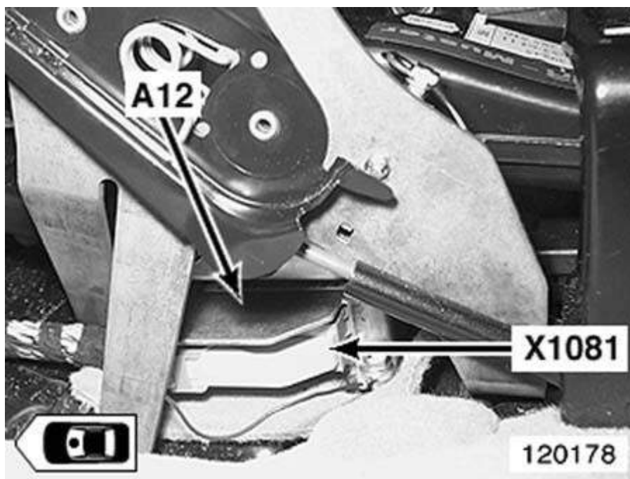
Fig. 20: Below Center Console
