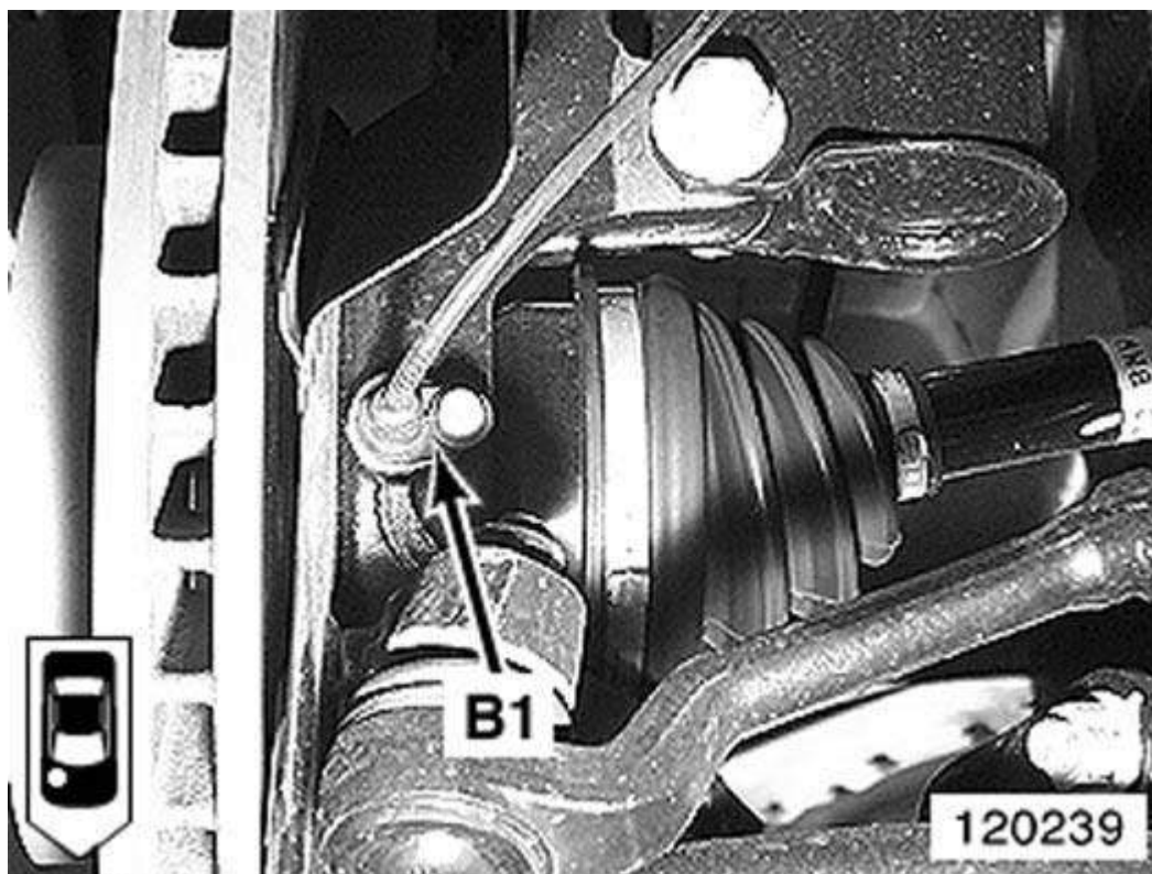
Fig. 27: Right Front Wheel
