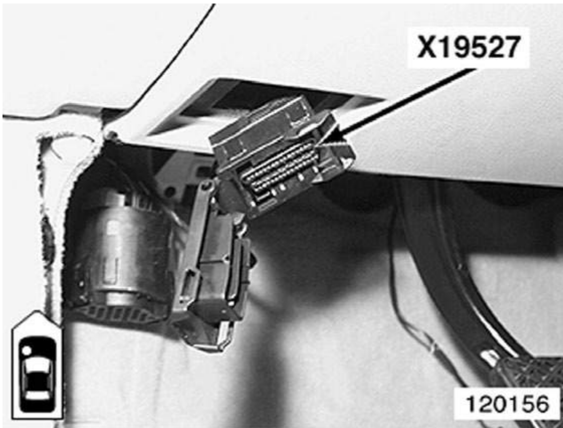
Fig. 9: Left Side Of Dash
