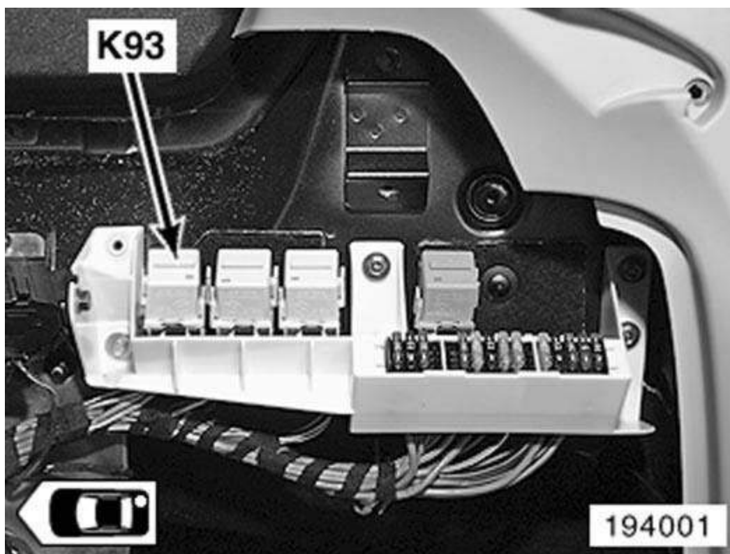
Fig. 48: Right Rear Of Luggage Compartment Courtesy of BMW OF NORTH AMERICA, INC.
