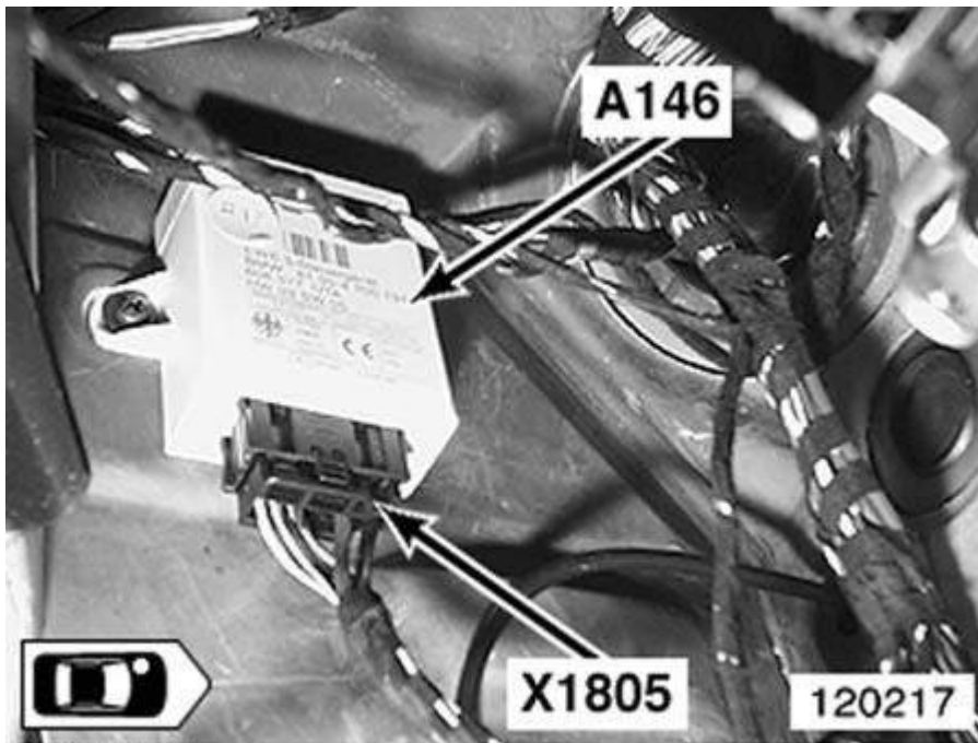
Fig. 24: Left Kick Panel
