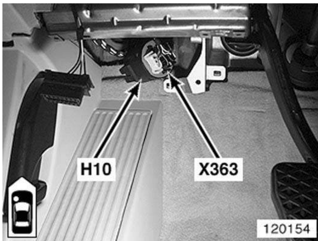
Fig. 41: Left Side Of Dash
