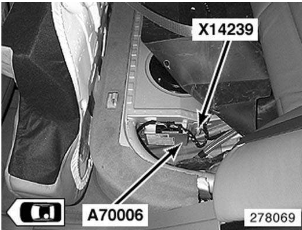
Fig. 26: Below Left Rear Seat
