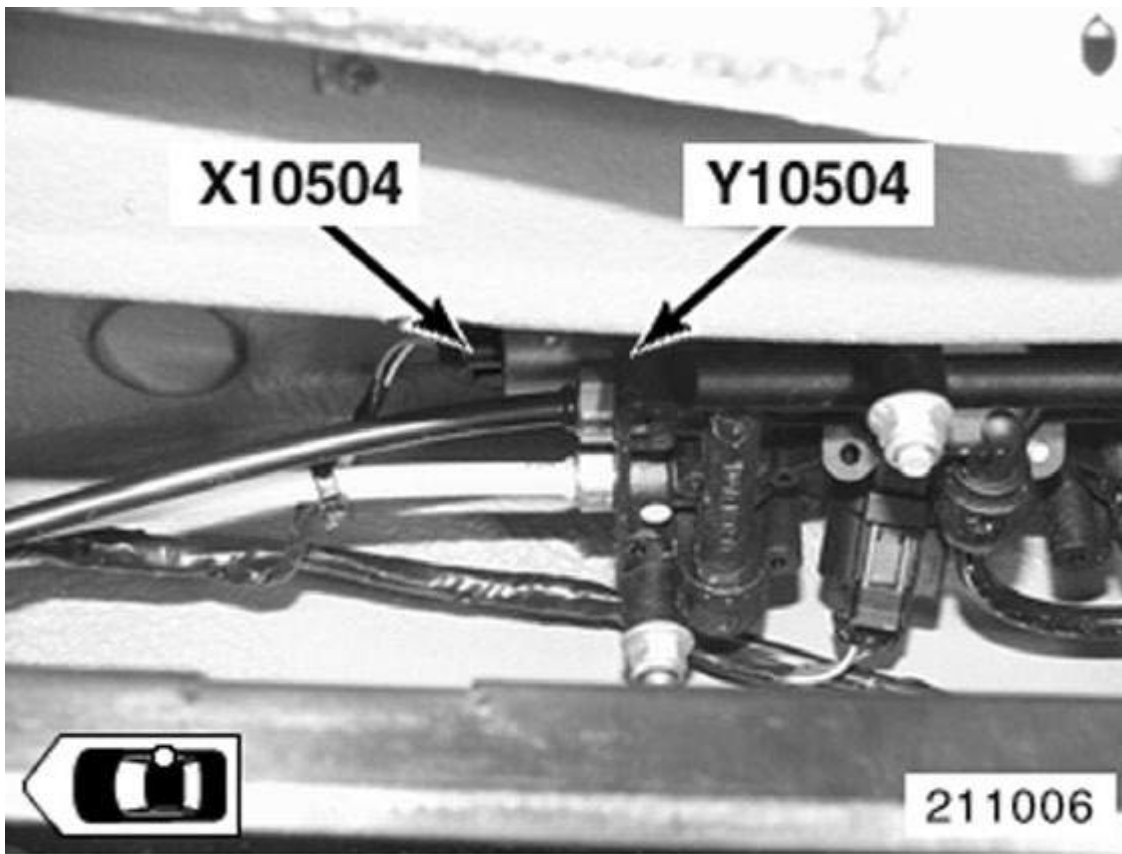
Fig. 60: Under Right Front Center Of Vehicle Courtesy of BMW OF NORTH AMERICA, INC.
