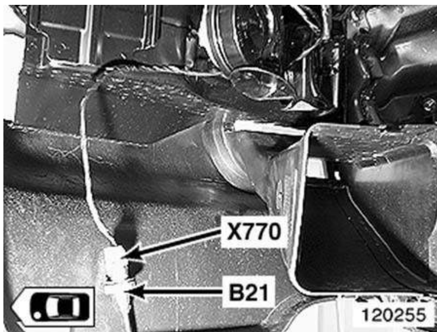
Fig. 34: Under Left Front Bumper
