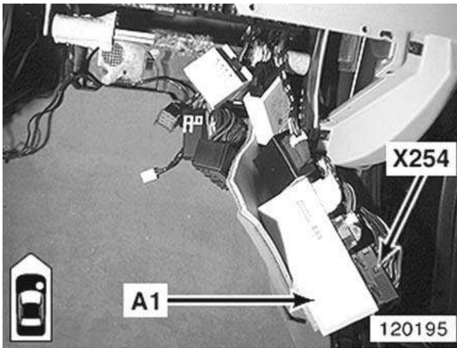
Fig. 18: Behind Glove Box
