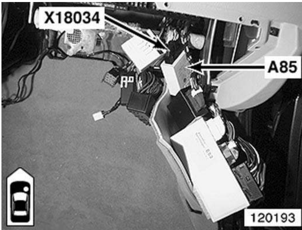
Fig. 22: Behind Glove Box
