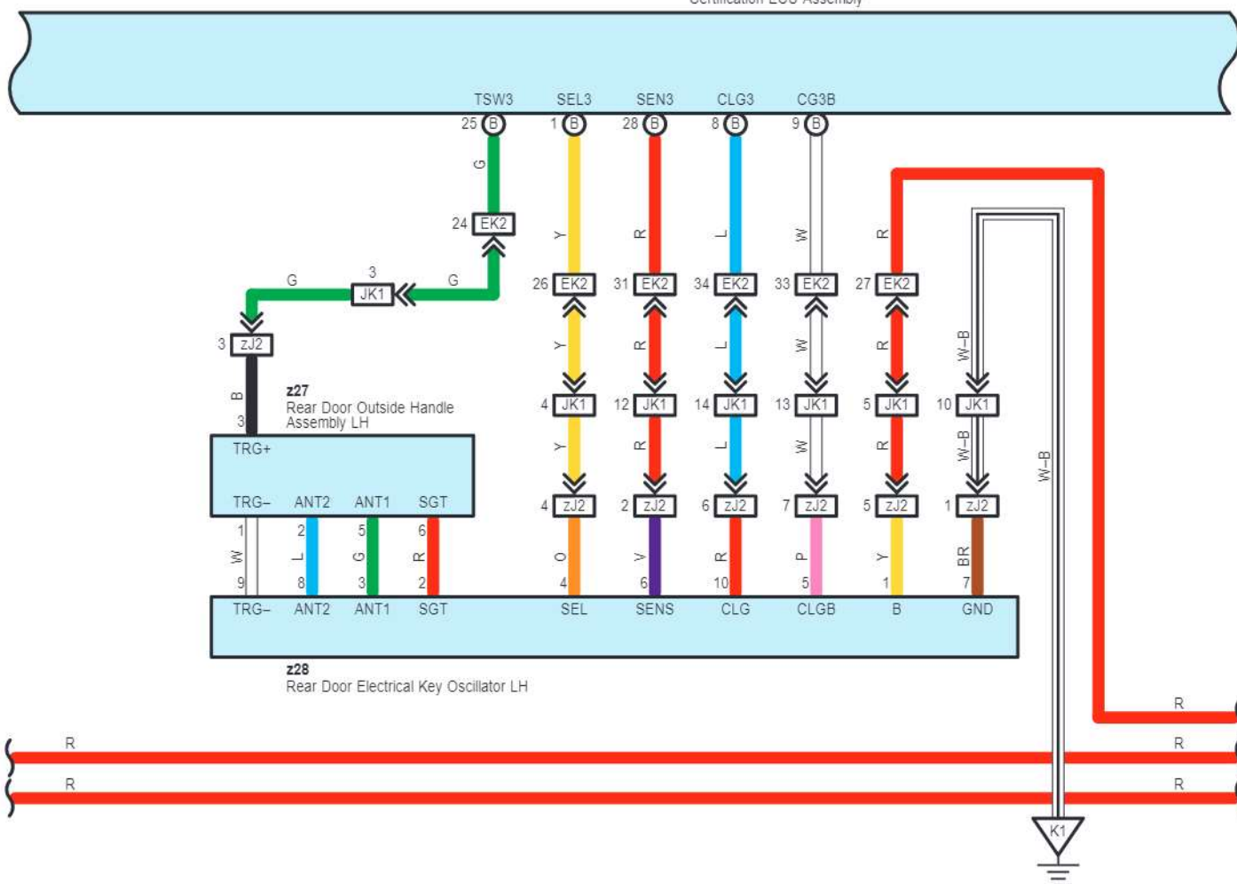
E29(A), E30(B) Certification ECU Assembly
