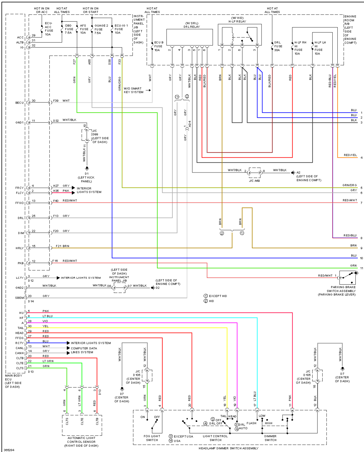
Fig. 48: Headlights Circuit (1 of 2)
