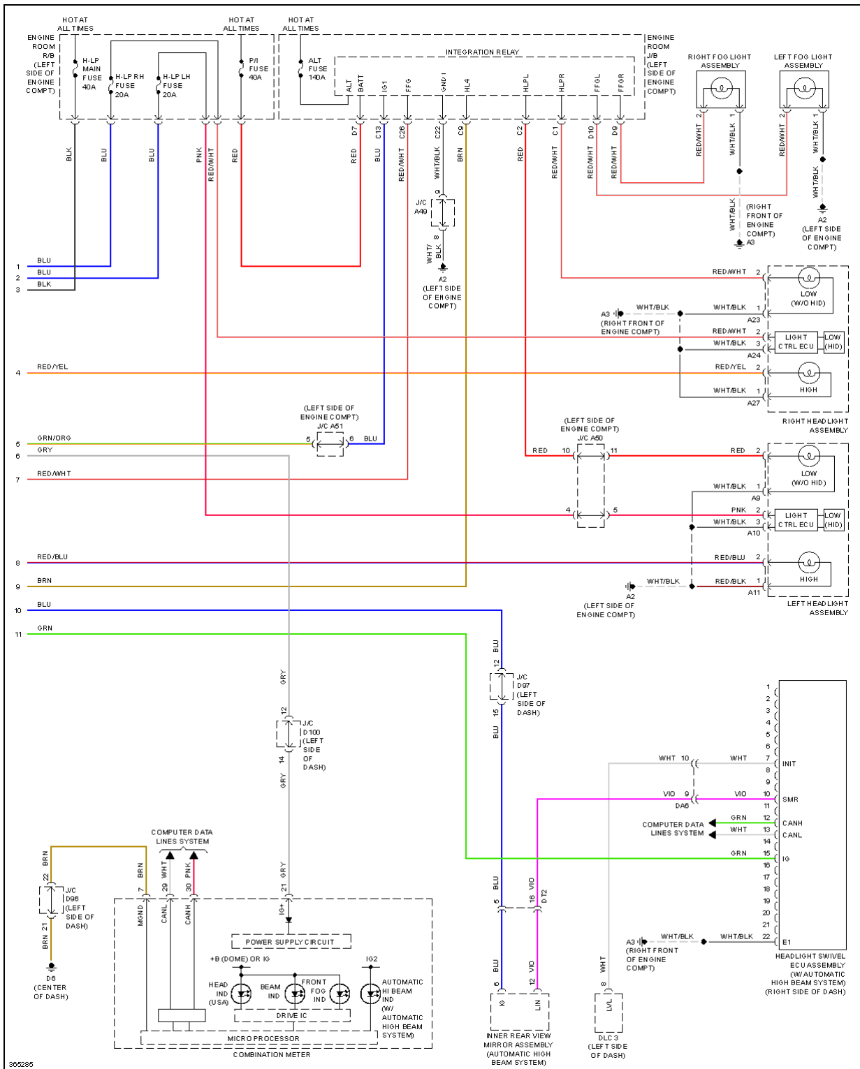
Fig. 49: Headlights Circuit (2 of 2)
