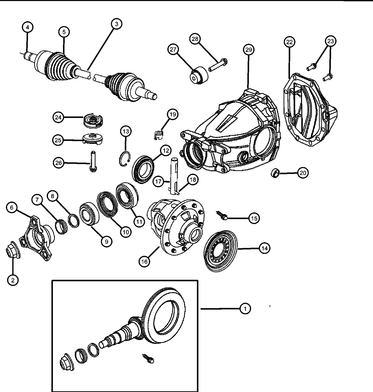
Housing and Differential with Internal Parts and Axle Shafts-[AWD] Figure 3-220
