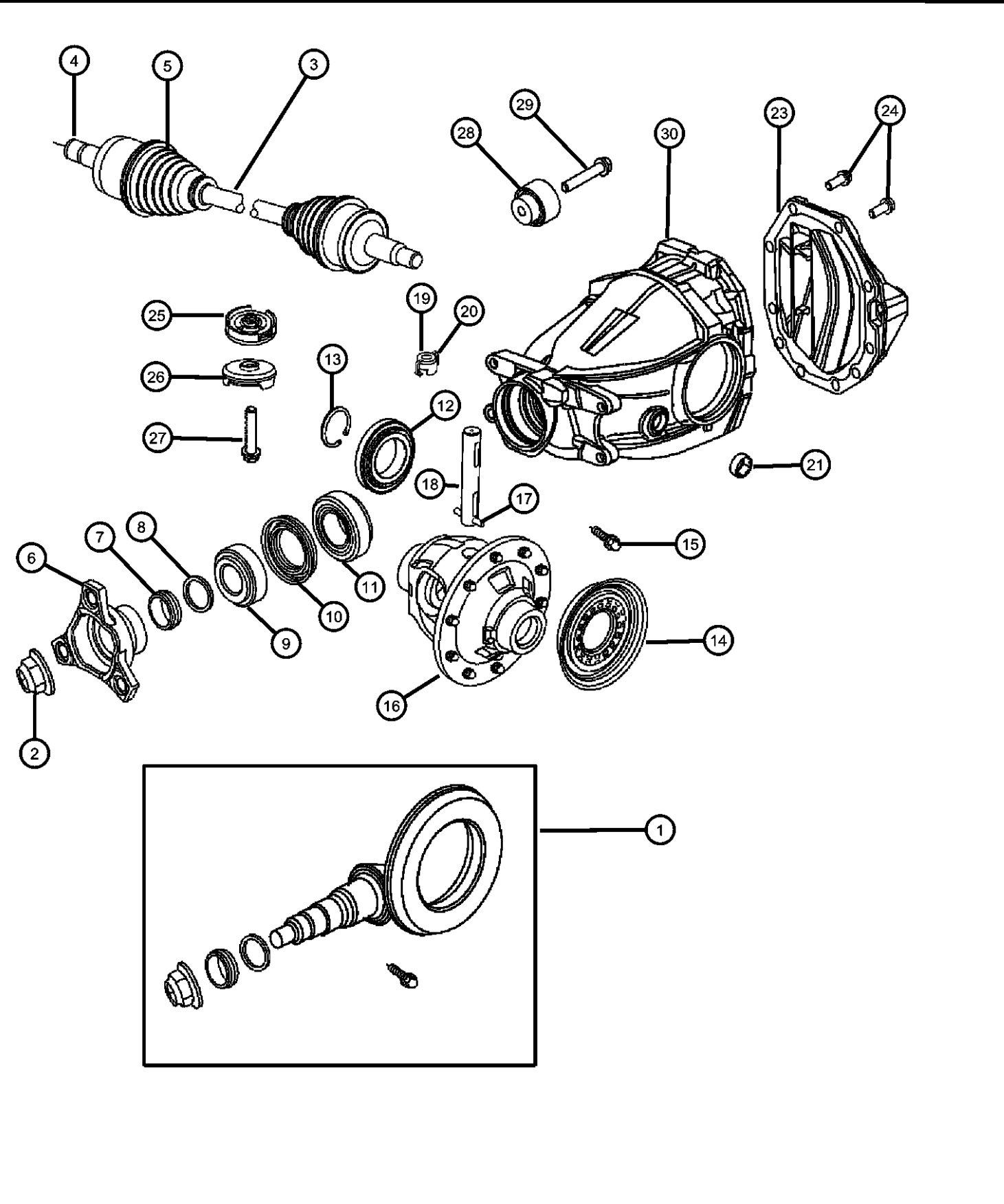
Housing and Differential with Internal Parts and Axle Shafts-[RWD] Figure 3-210
