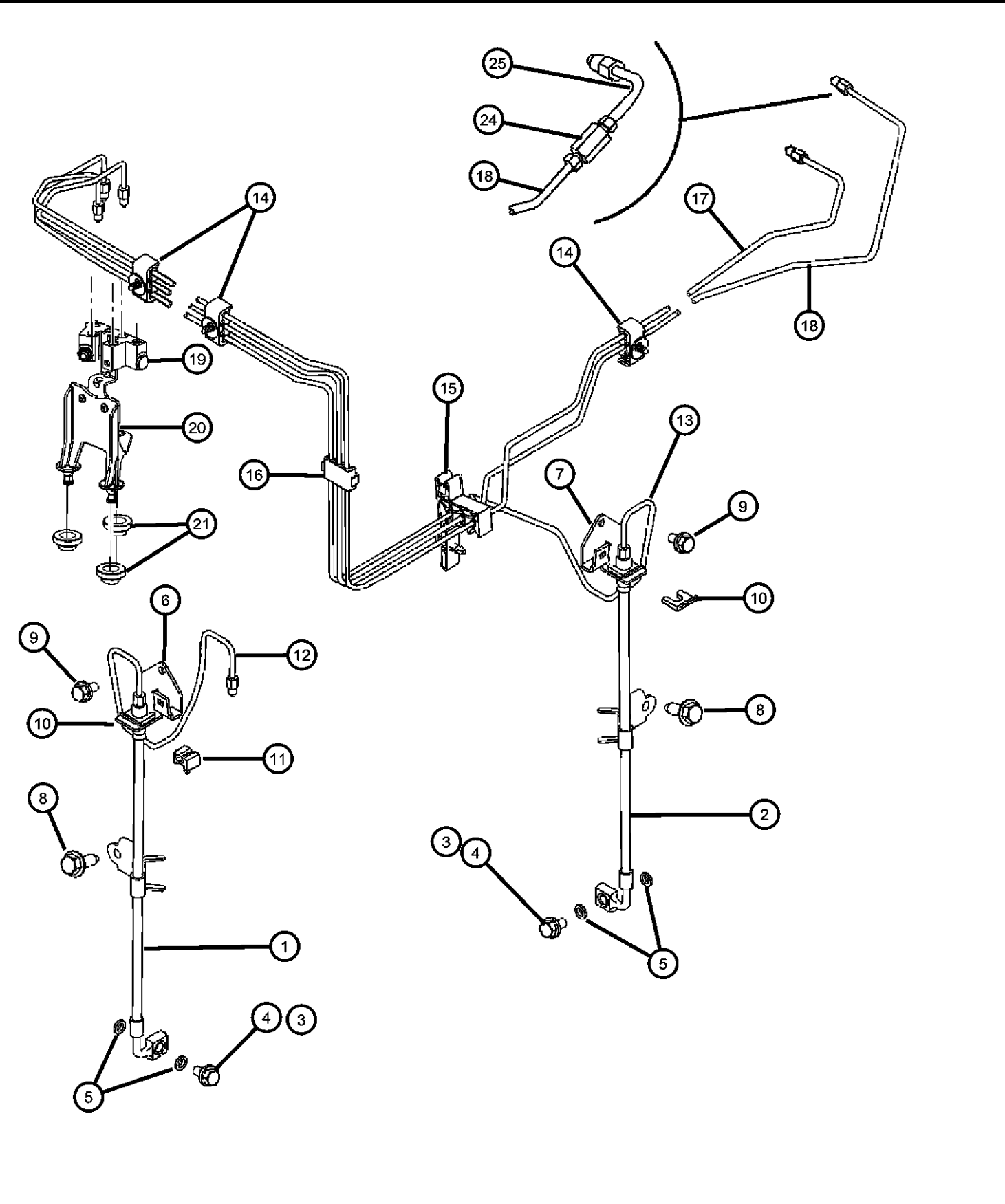
Lines and Hoses,Brake,Front Figure 5-510
