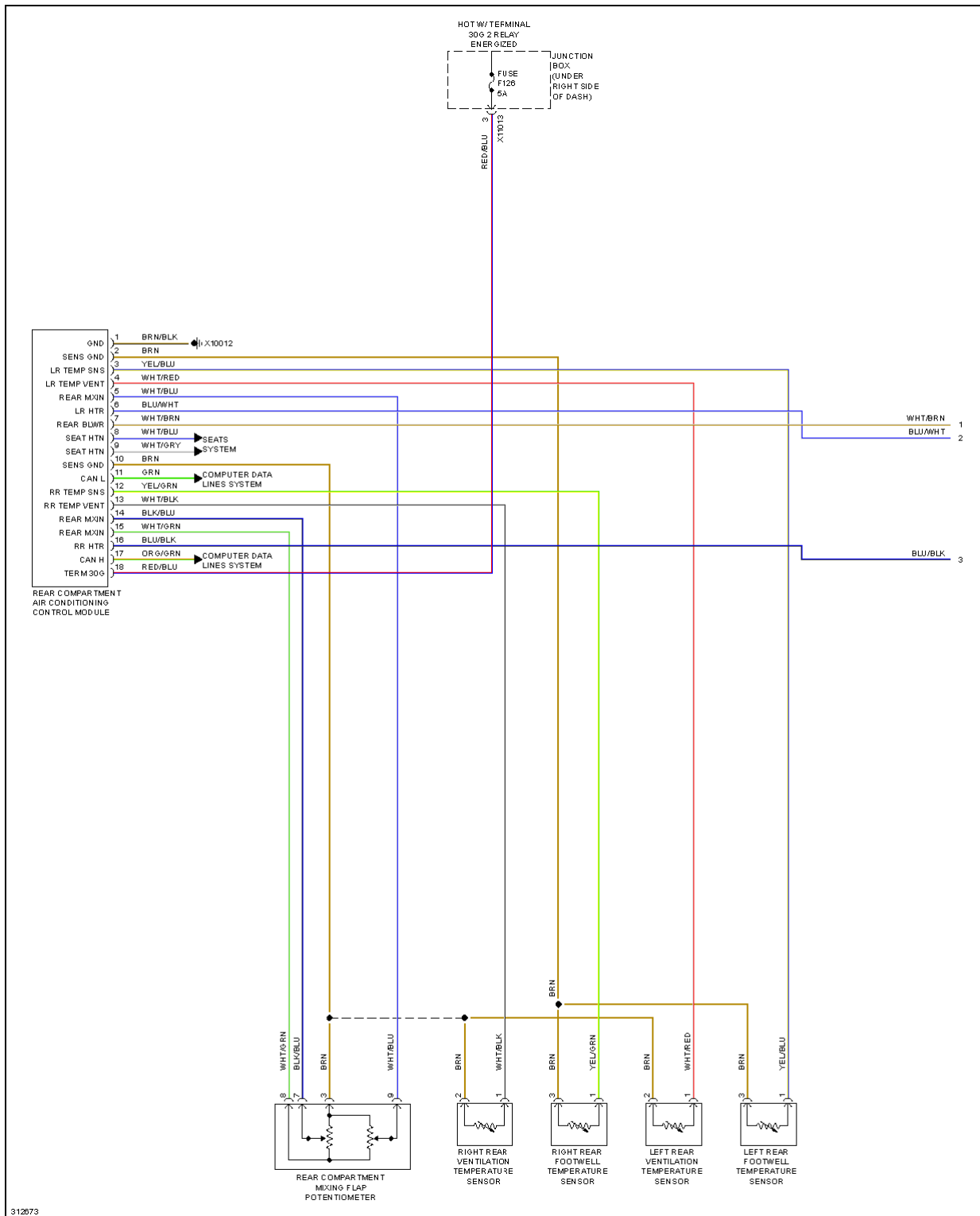
Fig. 11: Rear Heater & A/C Circuit (1 of 2)
