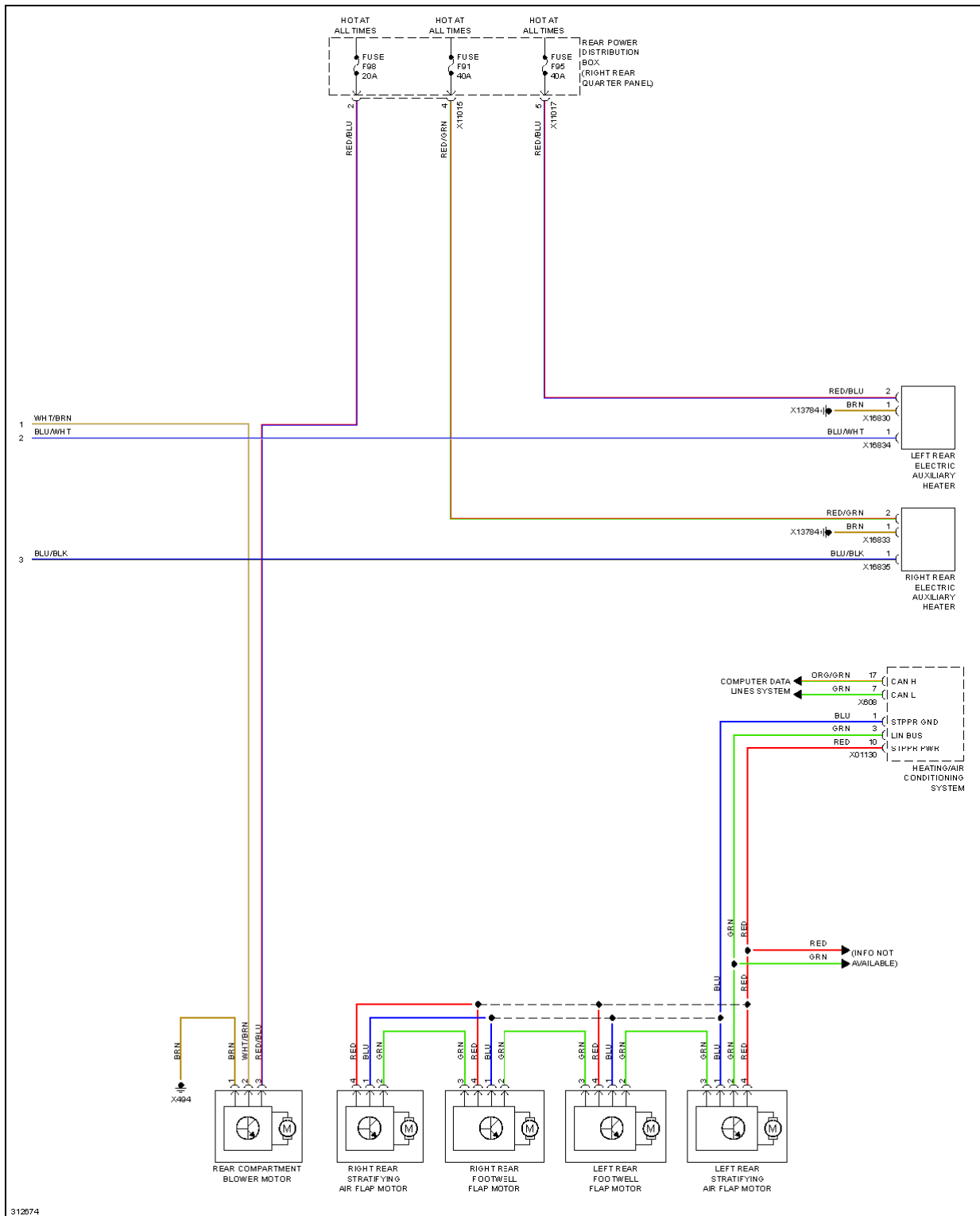
Fig. 12: Rear Heater & A/C Circuit (2 of 2)
